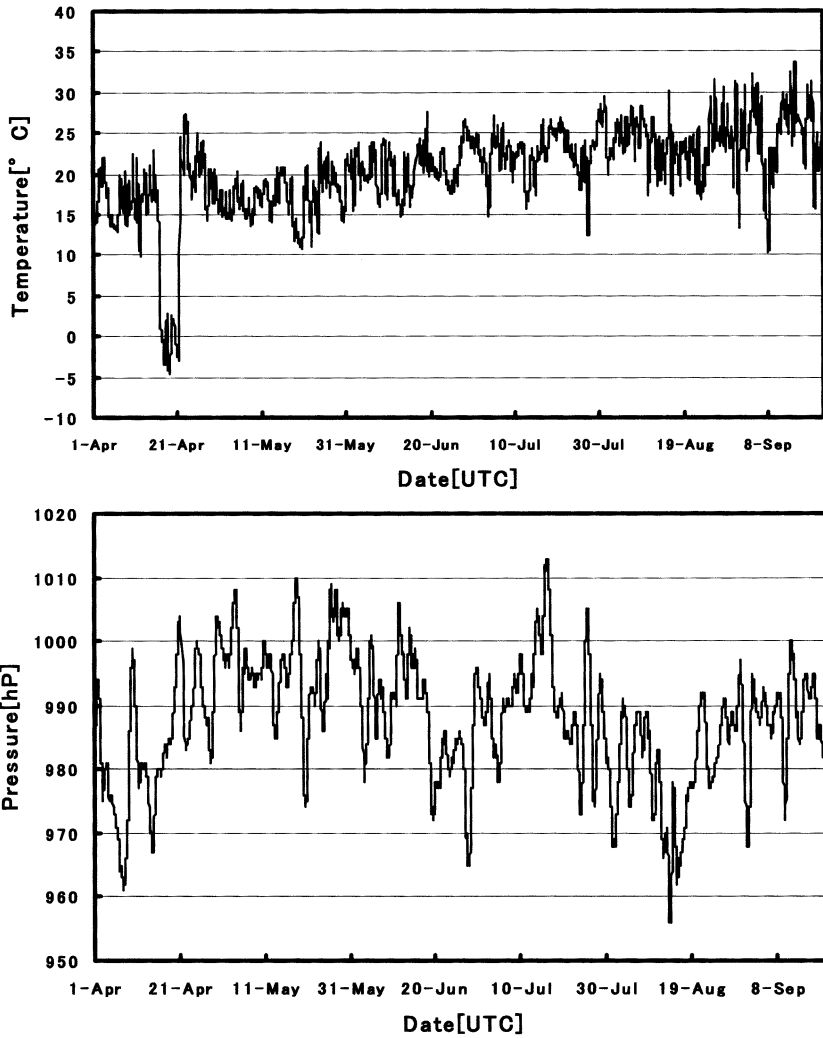
Fig. 18. Examples of the received data (above: temperature, below: pressure).
