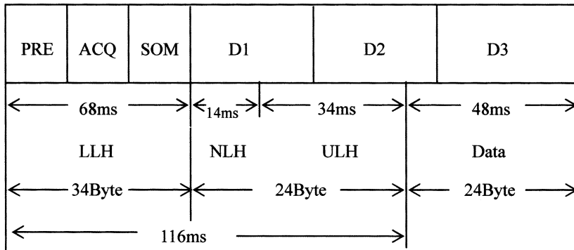
Fig. 14. Structure of the data packets used at the experiment.
