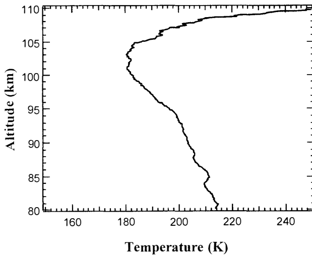
Fig. 5. Average night temperature profile for May 27–28, 2000.
