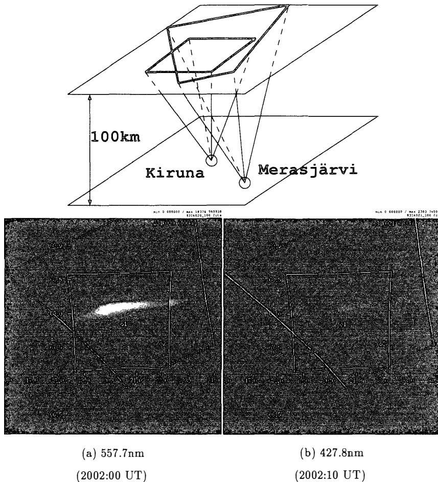
Fig. 6. The observed images projected at 100 km height. The upward direction of the paper is the geographic north.
