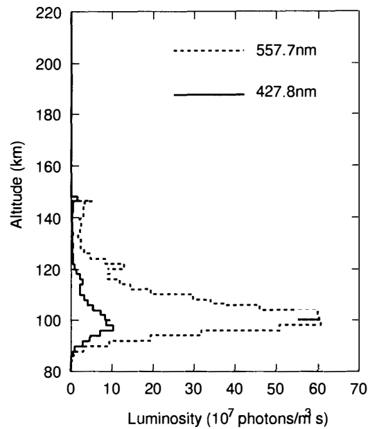
Fig. 8. Profiles of the reconstructed emission rate.
