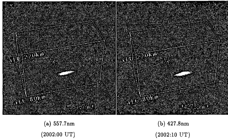
Fig. 7. Visualization of the reconstructed emission rate.
