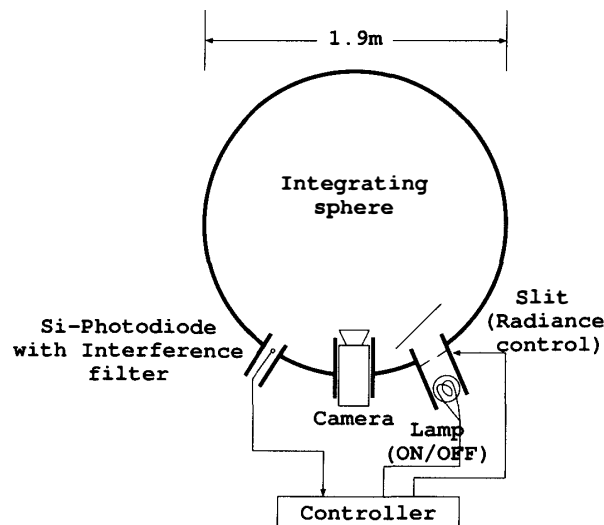
Fig. 2. The integrating sphere calibration standard (OL 462).
