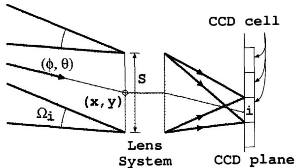
Fig. 1. Optical path to the cell i from column-like region.
