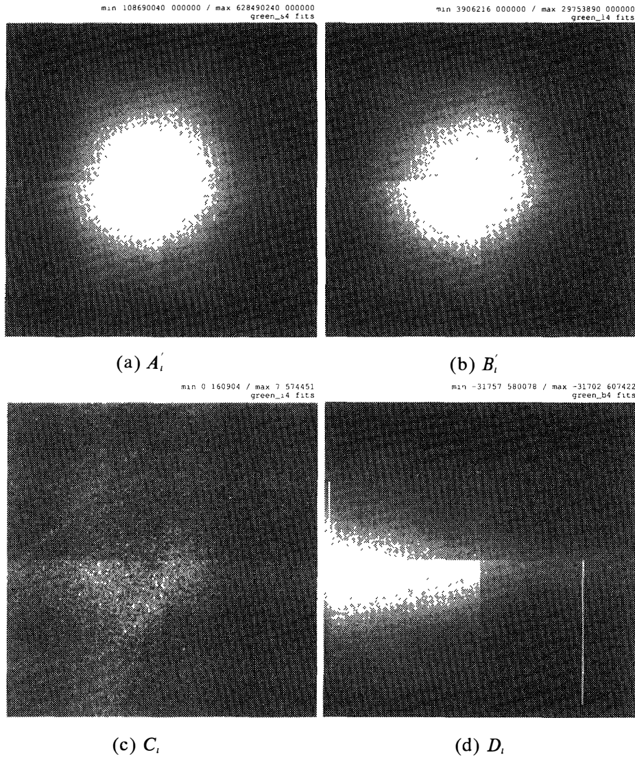
Fig. 4. The parameter image of the absolute calibration (557.7 nm).
