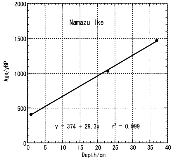
Fig. 2. Relationship between depth and age (conventional age) of sediment core of Namazu Ike (lake) at Skarvsnes in Syowa Station area.
