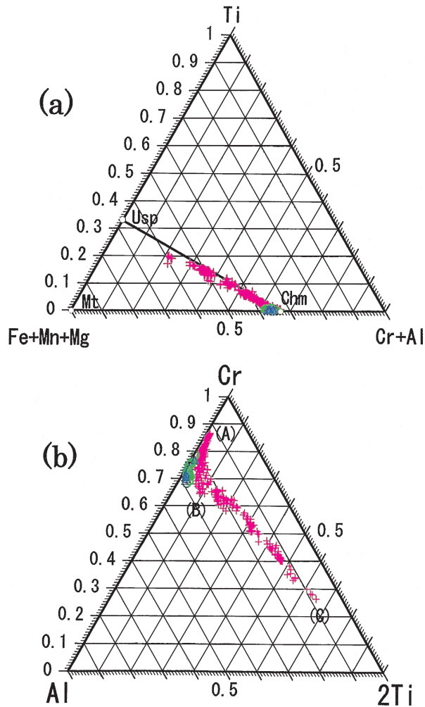
Fig. 3. Chromites are plotted in (a) Ti-(Fe+Mn+Mg)-(Cr+Al) and in (b) Cr-Al-2Ti in atomic ratios. Red symbol (chromite in contact with maskelynite), green circle (chromite in unusual inclusions, symplectic type), and blue triangle (chromite in unusual inclusions, non-symplectic type). The end components of chromite (Chm), ulvöspinel (Usp), and magnetite (Mt) are shown by open circles, and a solid solution between chromite and ulvöspinel is shown by a bold line in Fig. 3a. Cr-rich, Al-rich, and Ti-rich chromites are designated by (A), (B), and (C), respectively in Fig. 3b.
