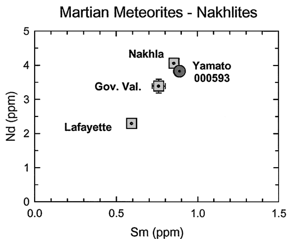
Fig. 5. Samarium versus neodymium abundance plot for nakhrites. Antarctic nakhlite Y000593 (circle) is the un-leached WR1 sample from this study. Literature data for non-Antarctic nakhrites are shown by squares. Y000593 has the same Sm and Nd abundances as Nakhla. Lower Rb, Sr and REE abundances in Lafayette may be the results of a higher degree of partial melting of the source, or of post-eruption of olivine accumulation.
