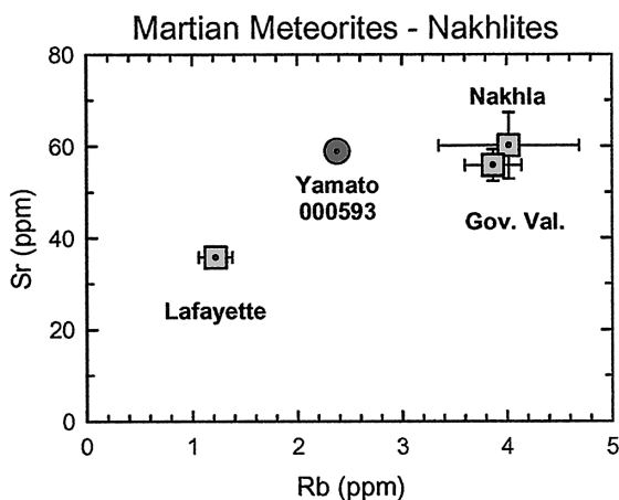
Fig. 2. Rubidium versus strontium abundance plot for nakhrites. Antarctic nakhlite Y000593 (circle) is the unleached WR1 sample from this study. Literature data for non-Antarctic nakhrites are shown by squares. Y000593 has the same Sr abundance as Nakhla and Governador Valadares but its Rb abundance is significantly lower than that in those two nakhrites. Lafayette has the lowest Rb and Sr among all nakhrites, perhaps due to its higher olivine and lower mesostasis content.
