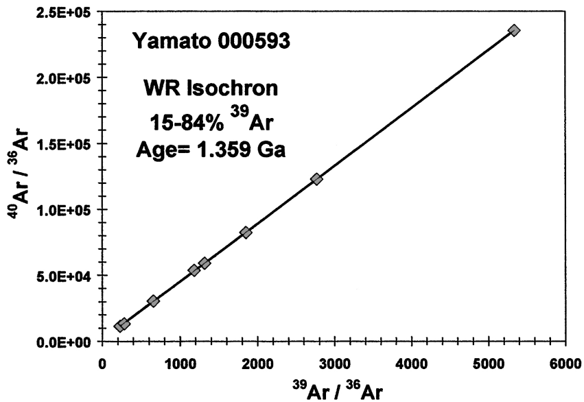
Fig. 9. Isochron plot of ^{40}\text{Ar}/^{36}\text{Ar} versus ^{39}\text{Ar}/^{36}\text{Ar} for nine extractions releasing 15–84% of the ^{39}\text{Ar} . The isochron age is 1.359 \pm 0.020 ( 2\sigma ) Ga and the ^{40}\text{Ar}/^{36}\text{Ar} intercept is 1502 \pm 159 . We interpret the isochron age as the most reliable ^{39}\text{Ar} - ^{40}\text{Ar} age of Y000593 (see text). Higher apparent ages shown in Fig. 8 for individual extraction temperatures indicate the presence of excess ^{40}\text{Ar} .
