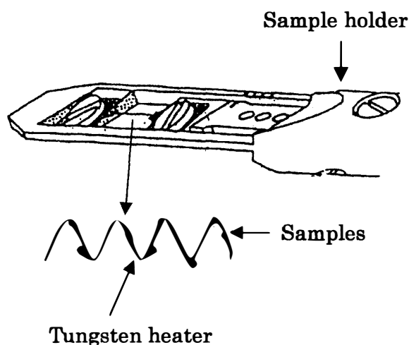
Fig. 2. Schematic representation of the sample holder used in the in-situ observation. QCC samples were directly mounted on the conical tungsten heater. Samples are shown by filled circles.
