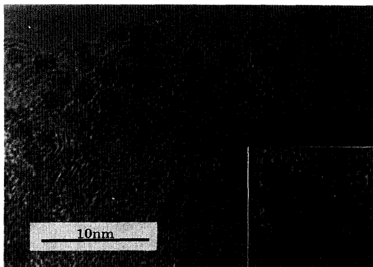
Fig. 5. HREM images of microdiamond appearing on the surface of QCC. The inset is the enlargement of a part of the black spots. The (111) lattice images of 0.206 nm which correspond to diamond can be clearly seen.
