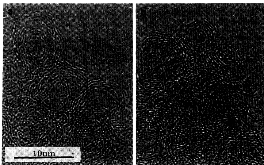
Fig. 3. HREM images of (a) the granular-QCC and (b) the dark-QCC. The materials are an aggregate of onion-like particles. EM images are shown on the same scale.
