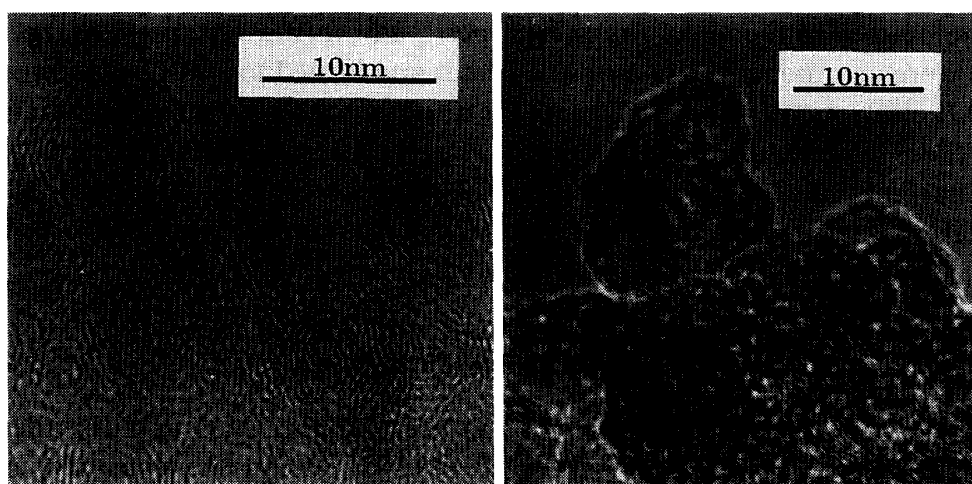
Fig. 4. HREM images of (a) dark-QCC heated for 40 min at 250°C in vacuum and (b) dark-QCC heated for 20 min at 500°C in vacuum. The peak position of sample (a) unchanged, and sample (b) shifted to 228 nm.
