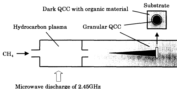
Fig. 1. Schematic representation of the experimental apparatus for producing QCC, which was previously reported by Sakata et al. (1994).
