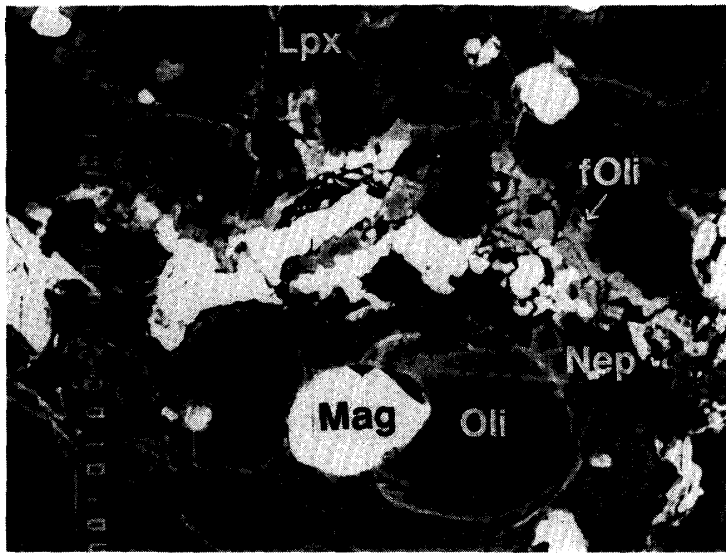
Fig. 1d. BSE image of an altered chondrule in Vigarano. Olivine phenocrysts (Oli) show distinct zoning. A Low-Ca pyroxene phenocryst (Lpx) is replaced by ferroan olivine (fOli) in the marginal parts. Plagioclase groundmass is also replaced by nepheline (Nep). Magnetite spherules (Mag) occur in this chondrule. Width of 120 microns.
