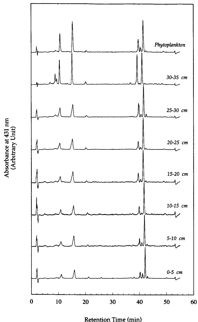
Fig. 3. Chromatogram profiles of ice algal and phytoplanktonic pigments. Chromatograms of ice algae are arrayed according to the vertical position in the sea ice. 0–5 cm represents the chromatogram of pigments extracted from ice algae collected from the bottom of the sea ice, and 30–35 cm is from uppermost level. The chromatograms were adjusted so that the height of Chl a would become the same in each chromatogram.
