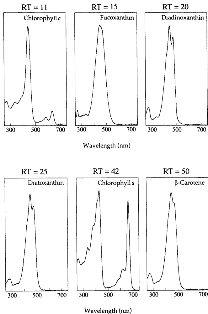
Fig. 2. Absorption pattern of each pigment separated from cultured Ch. gracilis in Fig. 1.
