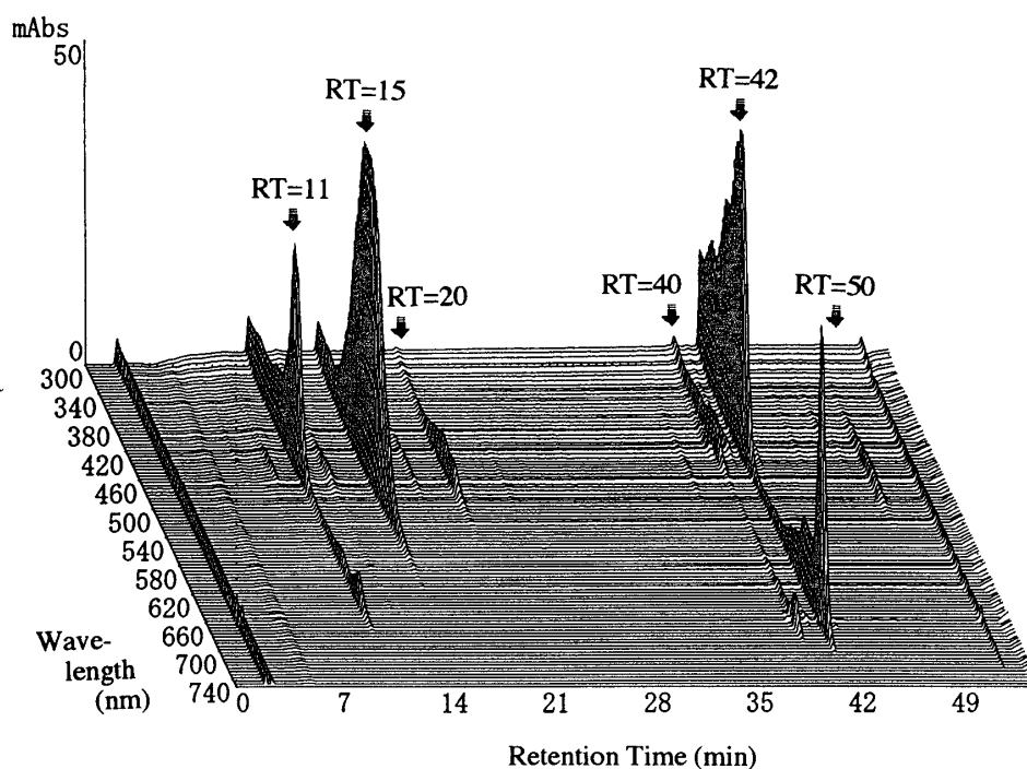
Fig. 1. A typical profile of HPLC analysis represented in 3-D view. Pigments extracted from cultured Chaetoceros gracilis were tested. See text for detail.
