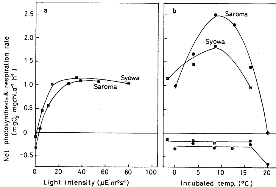
Fig. 4. A photosynthesis vs. light curve at 0°C (a), a photosynthesis vs. temperature curve under 57 \mu E m^{-2} s^{-1} , and a dark respiration vs. temperature curve (b) of ice algae in lagoon Saroma Ko. The curves at Syowa Station are from SATOH and WATANABE (1986).
