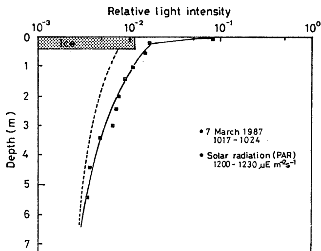
Fig. 2. Vertical profile of relative light intensity at Stn. A. The solid line represents the actual values obtained from ice hole. The dashed line indicates the values indirectly estimated in consideration of the light extinction by ice. See text for details.
