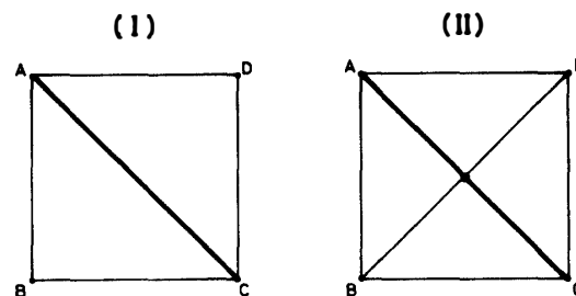
Fig. VI-9. The configuration of square strain grids.
