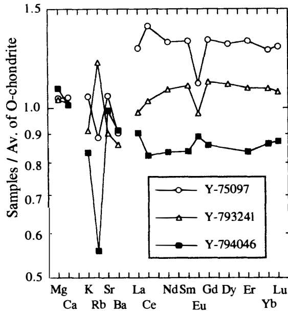
Fig. 3. Chondrite-normalized lithophile element patterns for host samples of the Y-75097 (L6), Y-793241 (L6) and Y-794046 (H5) chondrites. The Y-75097 meteorite has higher REE abundances, a minor positive Ce anomaly and a negative Eu anomaly. The Y-793241 meteorite shows a slightly fractionated REE pattern with a minor negative Eu anomaly. The weathered host specimen Y-794046 shows a depletion of Rb and K. Particularly, a large Rb depletion and the irregularity of La are unusual for an H-chondrite, and may be caused by the terrestrial weathering in Antarctica.
