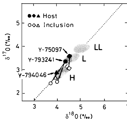
Fig. 1. Oxygen isotopic compositions of three inclusions and their host Yamato ordinary chondrites. Shaded areas indicate the ranges of the compositions of H-, L- and LL-chondrites. The hosts are L-chondrites, Y-75097 and Y-793241, and H-chondrite, Y-794046, whereas all three inclusions lie near the H-chondrite field. Data of Y-75097 and Y-793241 are from MAYEDA et al. (1987).
