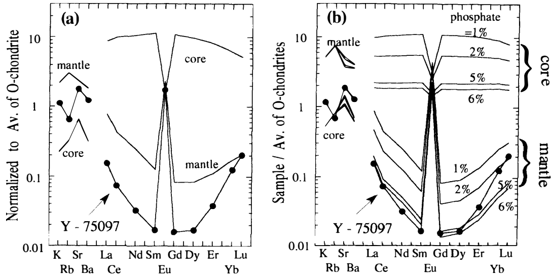
Fig. 5. Calculated REE patterns for the mineral assemblages of the core and mantle of the Y-75097 inclusion, based on solid/solid equilibrium partitioning (TORIGOYE et al. , 1993).
