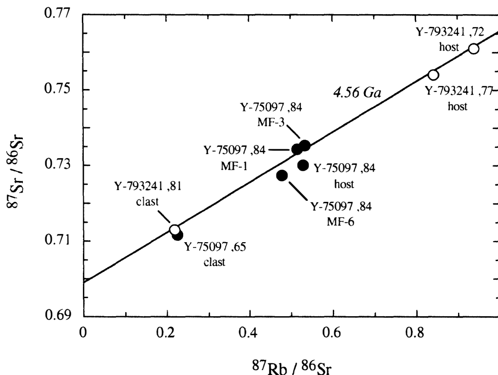
Fig. 2. ^{87}\text{Rb} - ^{87}\text{Sr} evolution diagram for the inclusions and the hosts of the Y-75097 (L6) and Y-793241 (L6) chondrites. The mineral separates (MF-1, MF-3 and MF-6) and a host specimen of Y-75097 do not form an isochron, indicating a late Rb-Sr isotopic perturbation, which also affected the Y-75097 inclusion. The data of two whole-rocks and the inclusion from Y-793241 form an isochron corresponding to an age of 4510 \pm 240 Ma and an initial ^{87}\text{Sr}/^{86}\text{Sr} ratio of 0.6985 \pm 0.0035 , indicating no perturbation since their early formation and/or metamorphism.
