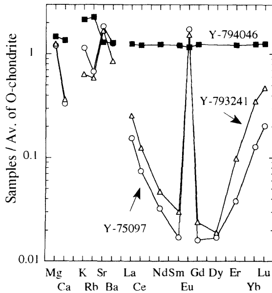
Fig. 4. Chondrite-normalized lithophile element patterns for inclusions from the Y-75097 (L6), Y-793241 (L6) and Y-794046 chondrites. The Y-75097 and Y-793241 inclusions show an extremely fractionated (V-shaped) REE pattern with middle REE depletion and large positive Eu anomaly. The Y-794046 inclusion has an unfractionated lithophile pattern except for its higher alkali contents ( \sim 2 \times O-chondrites).
