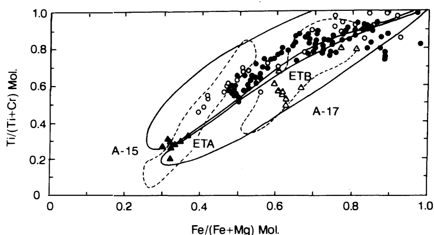
Fig. 5. Ti/(Ti+Cr) vs. Fe/(Fe+Mg) mol ratios for pyroxenes in Y-793169. Data from A-15 mare basalts and A-17 VLT basalts are from NIELSEN and DRAKE (1978). Open circles: Y-793169; solid circles: A-881757. ETA and ETB represent Groups A and B of EET87521 (BOESENBERG and DELANEY, 1992). Triangles (filled: Mg-rich and open: Fe-rich): Our data of EET87521.
