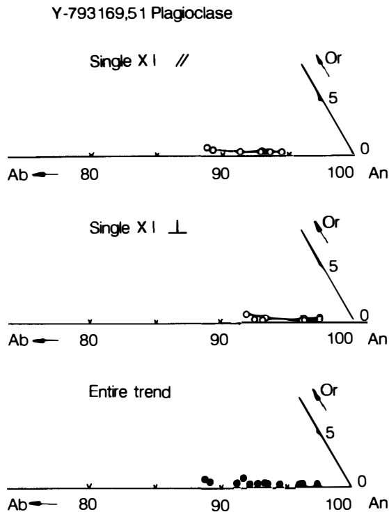
Fig. 3. A part of Or-Ab-An diagrams of plagioclase of Y-793169. Numbers are An and Or values in mole %.
