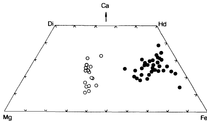
Fig. 4. (a) Pyroxene quadrilateral of A-881757 (present study), showing more Fe-rich trend than that of Y-793169. The circles connected by lines represent one traverse. (b) Summary of Y-793169 data. Open circles are Mg-rich cores and solid circles are Fe-rich areas.
