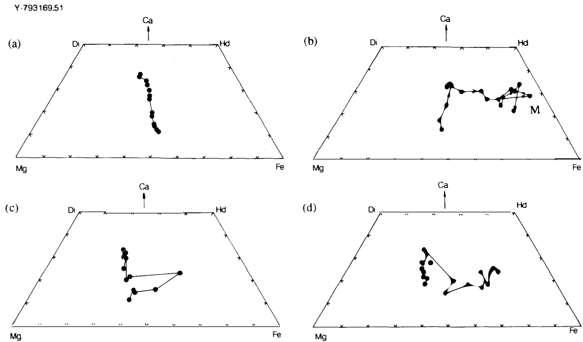
Fig. 2. Pyroxene quadrilaterals of Y-793169, showing chemical variations of some typical zoning trends. Subnumbers (a-d) refer to different single crystals. M: Mesostasis
