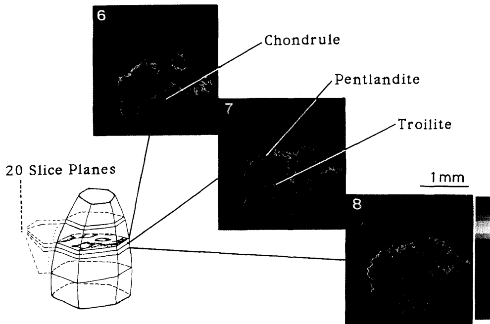
Fig. 3. Illustration of the Allende meteorite and CT images. The Allende meteorite was measured at 30 keV with twenty slice planes. The slice thickness was 37\ \mu\text{m} and the slice planes were spaced at 110\ \mu\text{m} intervals.
