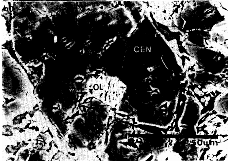
b. Clinoenstatite in a chondrule of ALH-764 showing weak Fe-Mg heterogeneity. Lines crossing the crystal from the upper right to the lower left are scratches of the section.
