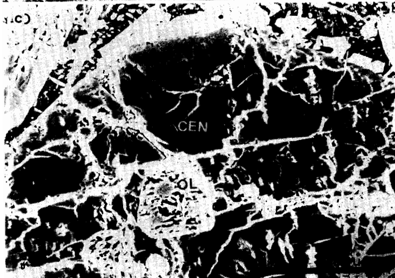
Fig. 1. Photomicrographs of the pyroxene textures under a SEM (BEI's) are arranged in the order of the petrologic types from type 3 to type 4. CEN=clinoenstatite. AUG=augite. PIG=pigeonite. OL=olivine. CHM=chromite. TR=troilite.
