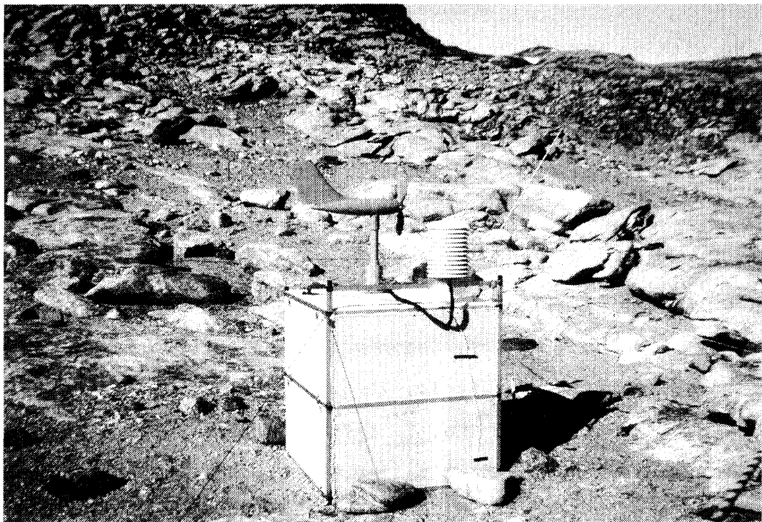
Fig. 2. Landscape around the unmanned observation station (MCS-4) toward the southeast.
