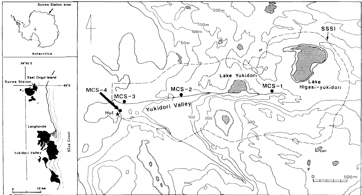
Fig. 1. Map showing the unmanned observation station at the Yukidori Valley, Langhovde.
