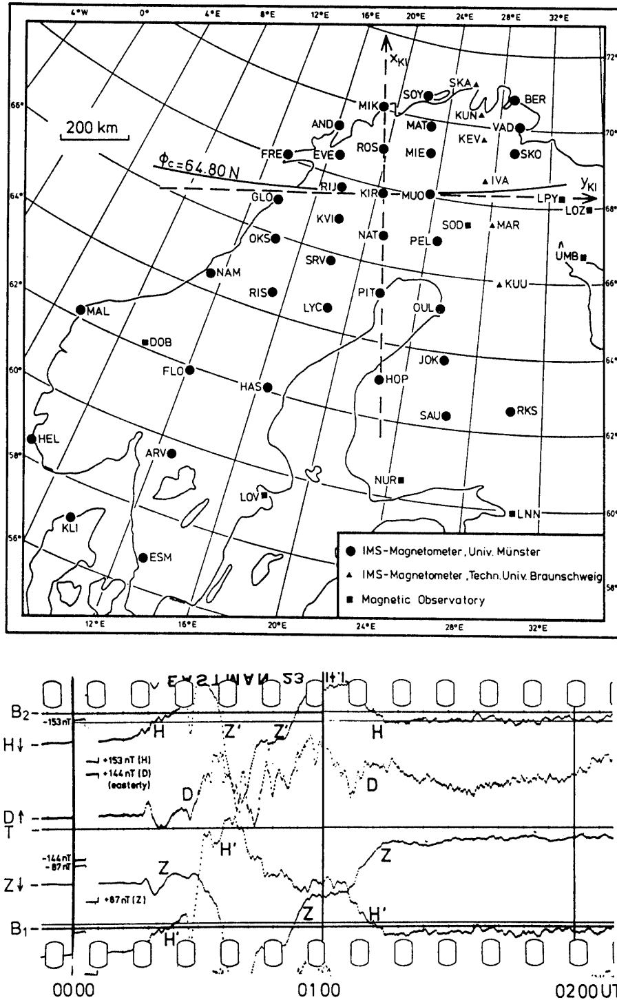
Fig. 1. Upper panel: Station map of the Scandinavian Magnetometer Array in geographic coordinates given by KÜPPERS et al. (1979). Solid curve through KIR shows 64.80N corrected geomagnetic latitude (GUSTAFFSON, 1970). Broken lines are the axes of the Kiruna system defined by KÜPPERS et al. (1979). Lower panel: Example of a film record from station EVE of the Scandinavian Magnetometer Array (KÜPPERS et al., 1979). Curves for the H-, D- and Z-components consist of dots optically recorded by every 10 sec (20 sec at some of the stations) exposure.
