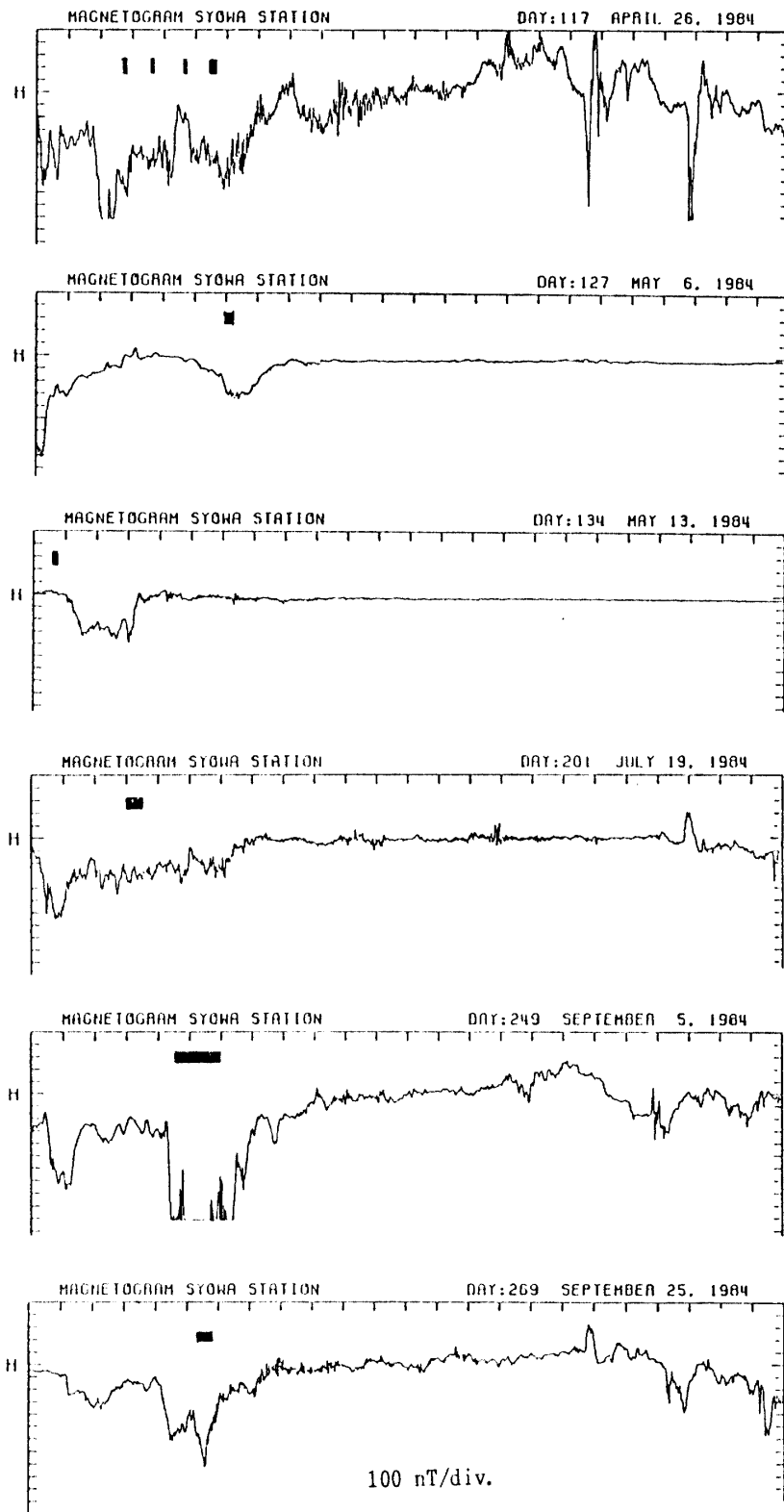
Fig. 3. Variations of geomagnetic H component at Syowa Station on the days of distinct type 5 echoes in 1984. The scale is 100 nT per division.
