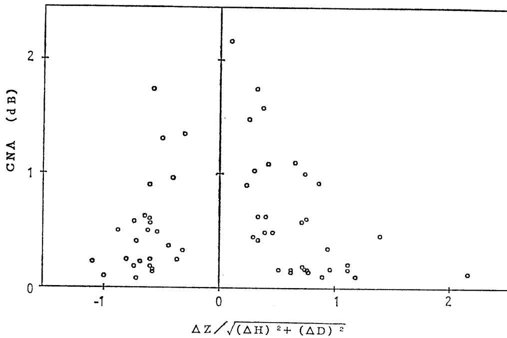
Fig. 8. Relation between intensity of CNA increase and the ratio of vertical component to horizontal component of magnetic preliminary impulse ( \Delta Z / \sqrt{(\Delta H)^2 + (\Delta D)^2} ) observed at Syowa Station.
