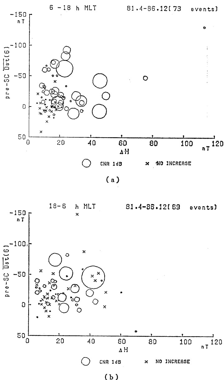
Fig. 5. (a) Diagram of intensity of CNA increase taking 6 hour-averaged Dst index ( \text{pre-SC } \overline{\text{Dst}}(6) ) in the ordinate and \Delta H at Honolulu in the abscissa with regard to 73 SC events occurred during 06-18 MLT from April 1981 to December 1986, and (b) diagram with regard to 69 SC events during 18-06 MLT of the same interval.
