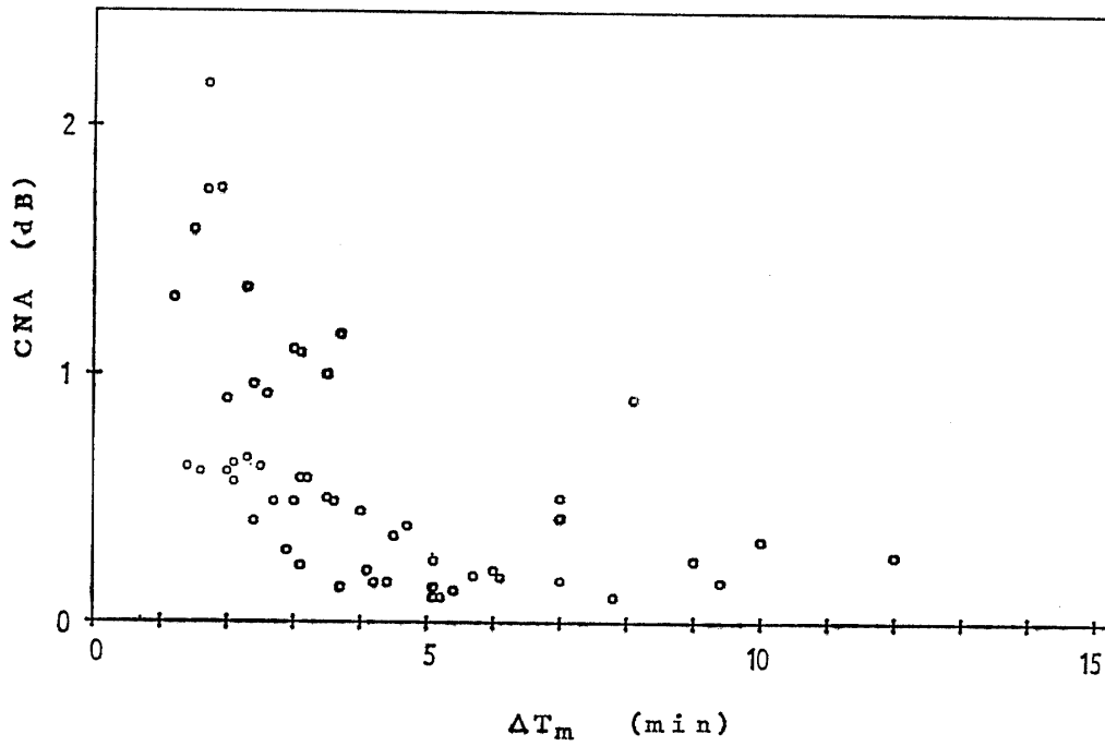
Fig. 7. Relation between intensity of CNA increase and the rise time of CNA ( \Delta T_m ) observed at Syowa Station.
