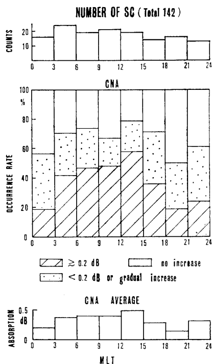
Fig. 2. Magnetic local time dependence of the occurrence of total 142 SC's observed at Syowa Station (top panel), the occurrence rate for each type of CNA increase (middle panel), and the average intensity of CNA (bottom panel).
