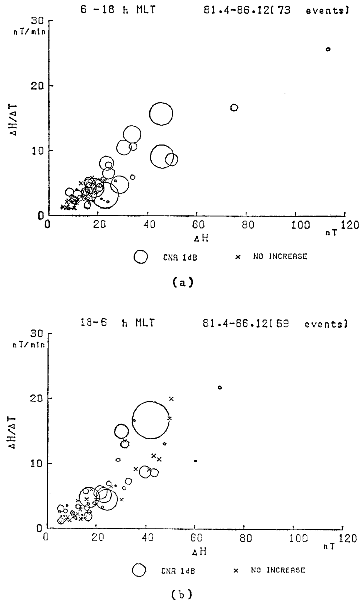
Fig. 6. (a) Diagram of intensity of CNA increase taking the ratio of SC amplitude to rise time ( \Delta H/\Delta T ) at Honolulu in the ordinate and \Delta H in the abscissa with regard to 73 SC events occurred during 06-18 MLT from April 1981 to December 1986, and (b) diagram with regard to 69 SC events during 18-06 MLT of the same interval.
