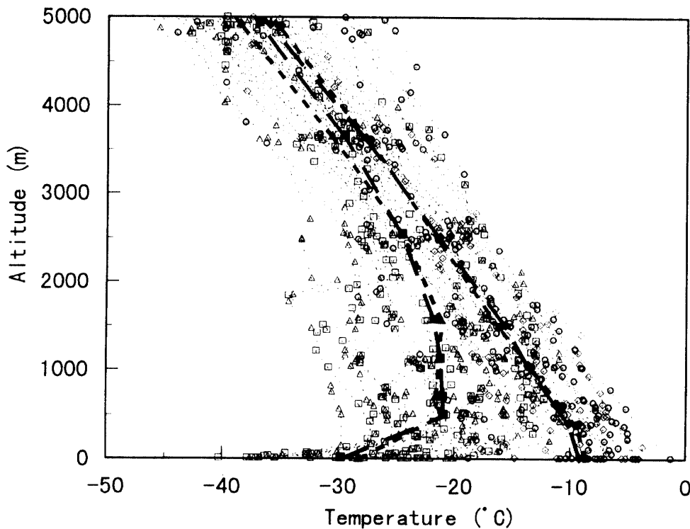
Fig. 3. Variations of vertical temperature profiles above Syowa Station. Temperatures on the standard and the significant levels are shown by different symbols: the beginning (□) and end (◇) of warming events, and the beginning (○) and end (△) of cooling events. Composite profiles compiled from only standard level data are shown by thick broken lines for warming events and thick dotted lines for cooling events, with black symbols for every case.
