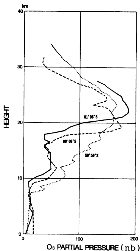
Fig. 7. Vertical profiles of ozone partial pressure in the region from the total ozone maximum point to Syowa Station. Vertical profiles at 59^{\circ}59'S , 89^{\circ}35'E (dotted line), 61^{\circ}06'S , 42^{\circ}18'E (solid line), and 69^{\circ}00'S , 39^{\circ}35'E (dashed line, at Syowa Station) are illustrated.
