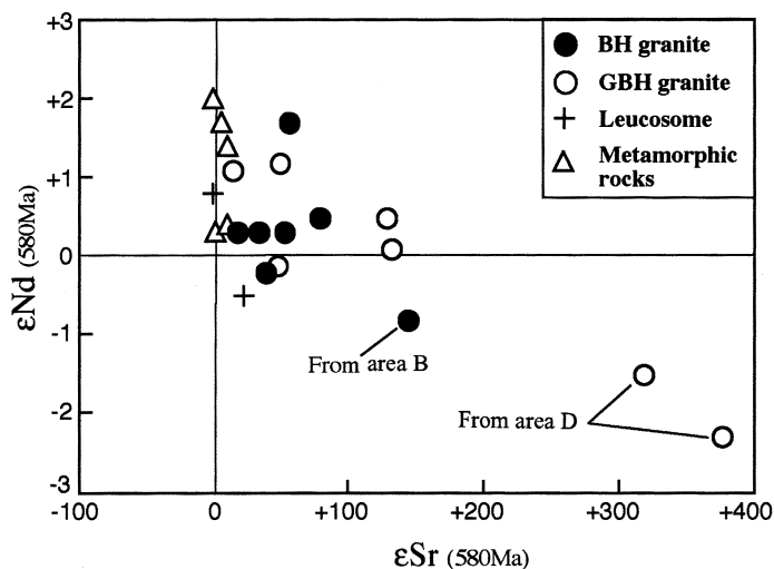
Fig. 8. \epsilon Sr_{580Ma} versus \epsilon Nd_{580Ma} diagram.
