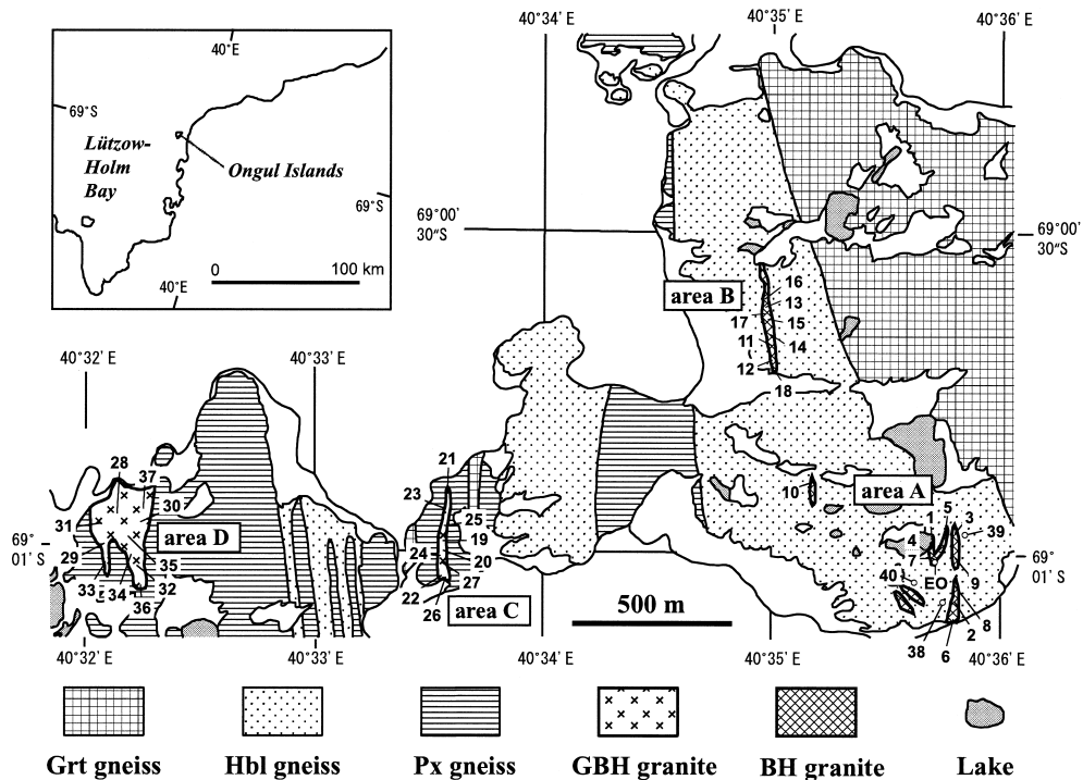
Fig. 1. Geological map of a part of the Ongul Islands simplified from Ishikawa et al. (1994). Grt, garnet; Hbl, hornblende; Px, pyroxene; GBH, garnet biotite hornblende; BH, biotite hornblende. EO is sampling site of 80EO125 discussed by Shibata et al. (1985, 1986). Numbers indicate sampling sites for analyzed rocks of the same number in Table 1.
