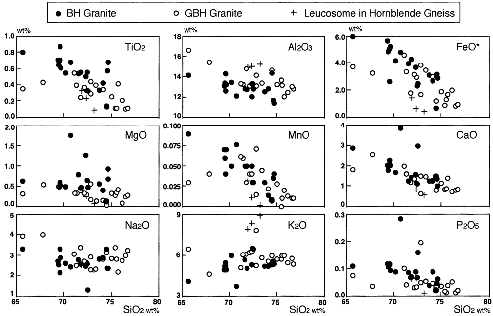
Fig. 5. Harker diagrams for major elements. FeO^* = FeO + 0.9Fe_2O_3 .
