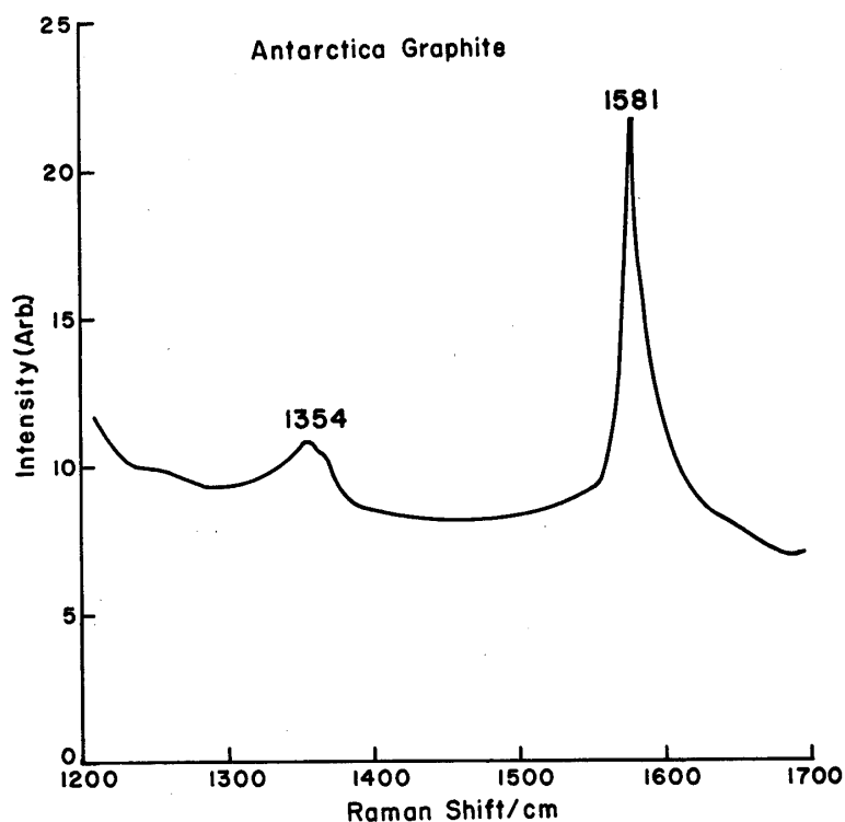
Fig. 3. First order Laser Raman Spectra of the graphite sample from Schirmacher Oasis, East Antarctica. The peaks 1581\text{ cm}^{-1} (G), and 1354\text{ cm}^{-1} (D) correspond to well-ordered and disordered Raman peak of graphite respectively.
