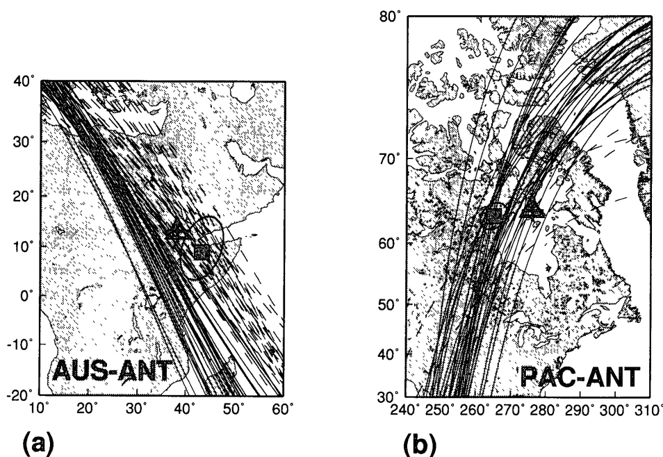
Fig. 11. Pole locations of the relative plate motions and meridian great circles which are perpendicular to slip vectors at epicenters. Crosses are pole locations by NUVEL1; solid squares are pole locations based on the GPS (LARSON et al. , 1997). Open triangles are locations of NUVEL-G (DEMETTS et al. , 1993), in which all slip vectors are excluded. Ellipses show error estimation for geodetic pole locations. (a) AUS-ANT case, (b) PAC-ANT case.
