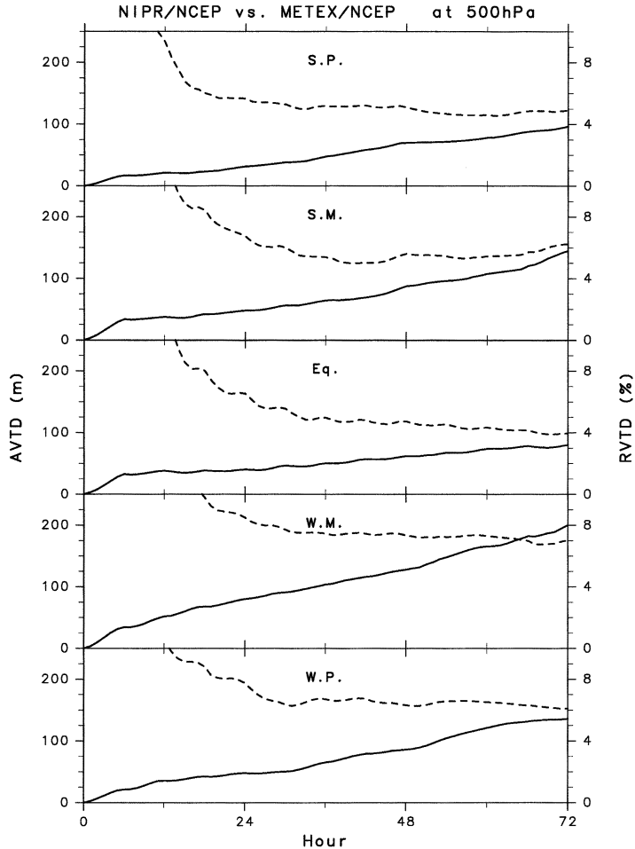
Fig. 3. The same as Fig. 2 but for AVTDs (solid) and RVTDs (dashed).
