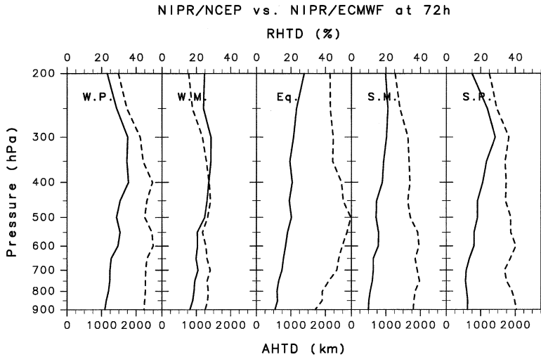
Fig. 8. The same as Fig. 4 but for NIPR/NCEP vs. NIPR/ECMWF.
