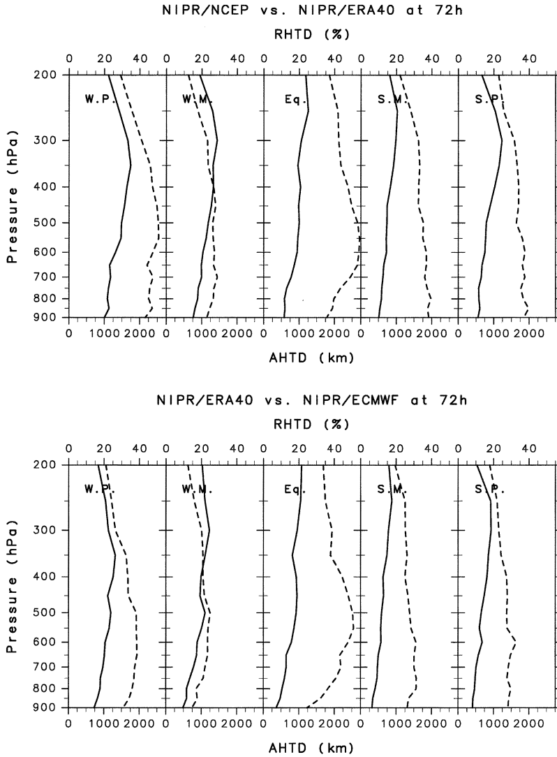
Fig. 10. The same as Fig. 4 but for (top) NIPR/NCEP vs. NIPR/ERA40 and (bottom) NIPR/ERA40 vs. NIPR/ECMWF.
