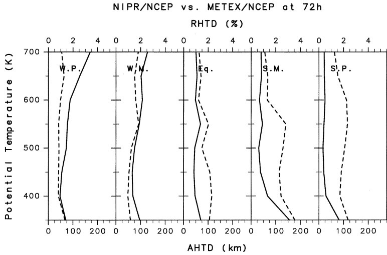
Fig. 6. The same as Fig. 4 but for isentropic trajectories as a function of potential temperature.
