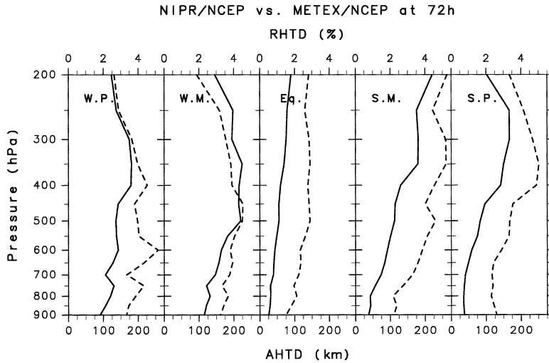
Fig. 4. AHTDs (solid) and RHTDs (dashed) at 72h for kinematic trajectories resulting from NIPR/NCEP vs. METEX/NCEP in five latitude regions as a function of initial pressure.
