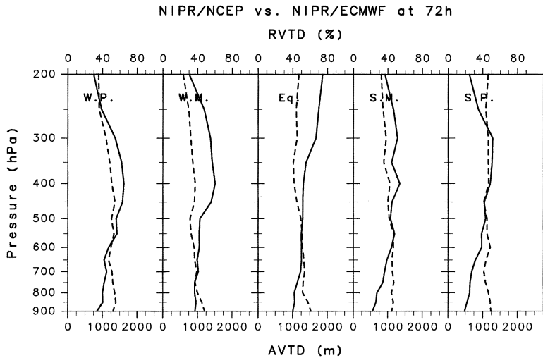
Fig. 9. The same as Fig. 5 but for NIPR/NCEP vs. NIPR/ECMWF.
