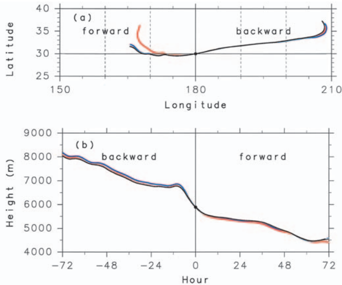
Fig. 1. (a) Horizontal map and (b) time change of heights of the forward and backward kinematic trajectories calculated with the NIPR model (blue), METEX (red), and HYSPLIT4 (black), starting from 180°E, 30°N at 500 hPa at 0000 UTC on July 10, 1998. Closed circles represent the initial positions of the trajectories.
