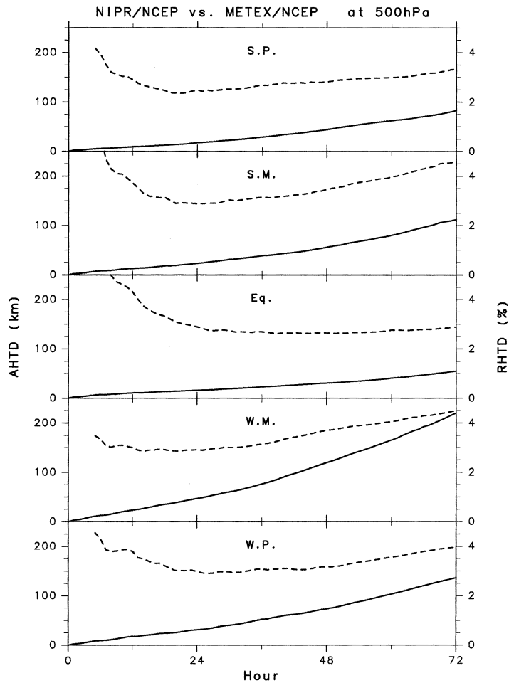
Fig. 2. AHTDs (solid) and RHTDs (dashed) for kinematic trajectories starting at 500 hPa, resulting from NIPR/NCEP vs. METEX/NCEP in five latitude regions, as a function of trajectory period.
