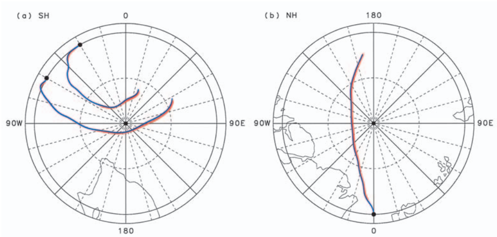
Fig. 7. Isentropic trajectories at 500 K, which passed (a) south of 87.5°S and (b) north of 87.5°N. Blue and red lines represent the trajectories calculated with the NIPR model and METEX, respectively. Solid circles show the initial positions. Solid and dashed latitude lines represent 80° and 85° latitudes, respectively.
