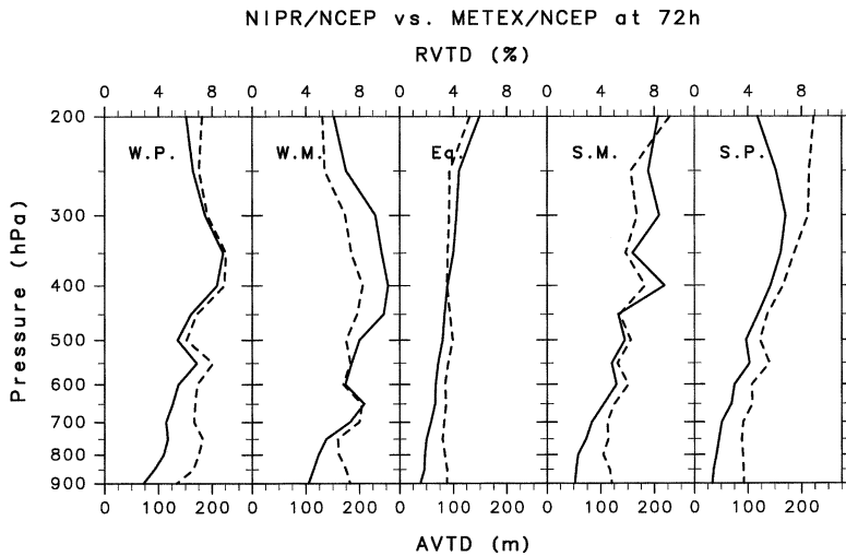
Fig. 5. AVTDs (solid) and RVTDs (dashed) at 72h for kinematic trajectories resulting from NIPR/NCEP vs. METEX/NCEP in five latitude regions as a function of initial pressure.
