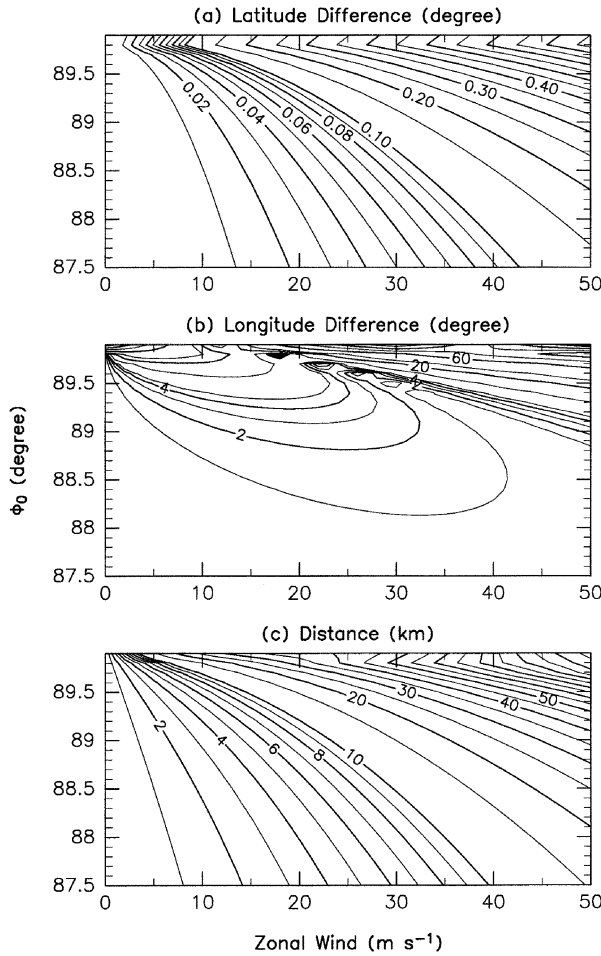
Fig. A1. (a) Latitude difference (degrees), (b) longitude difference (degrees), and (c) distance (km) between (\lambda_1, \phi_1, X_1, Y_1) and (\lambda_2, \phi_2, X_2, Y_2) as a function of zonal wind ( \text{m s}^{-1} ) and \phi_0 (degrees) for v=10 \text{ m s}^{-1} .
