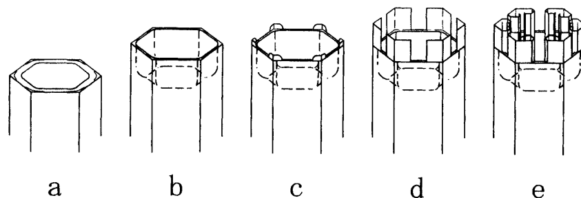
Fig. 7. Growth process of branches of a needle ice crystal growing in air at 10^5 Pa at -7^{\circ}\text{C} and at about water saturation.
