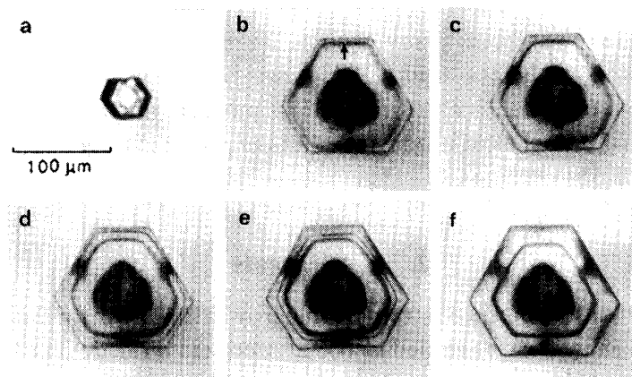
Fig. 2. Ice crystal growing in air at 10^5 Pa at -7^\circ\text{C} and at about 6% supersaturation. (a) 0, (b) 3.0, (c) 3.3, (d) 3.8, (e) 4.0 and (f) 5.0 min.
