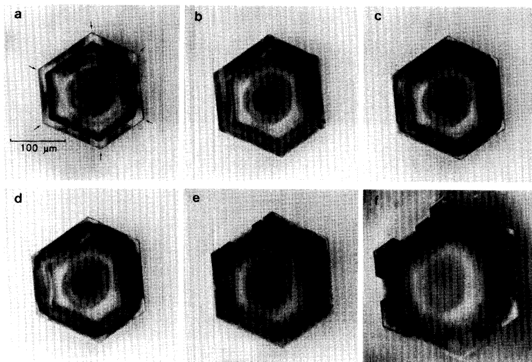
Fig. 3. Further growth of the same ice crystal as shown in Fig. 2. (a) 0, (b) 0.5, (c) 1.0, (d) 2.0, (e) 7.0 and (f) 12 min.
