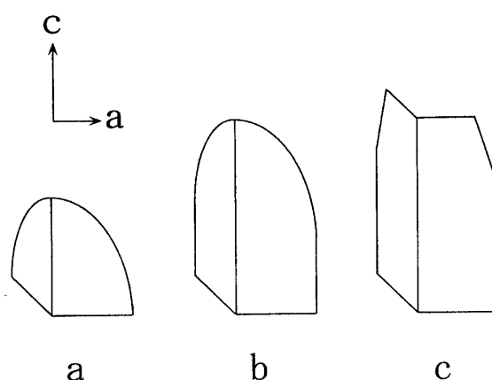
Fig. 8. Growth process of a branch of a needle ice crystal growing in air at 10^5 Pa at -7^\circ\text{C} and above water saturation.
