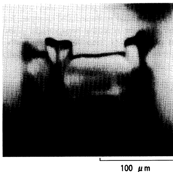
Fig. 4. Ice crystal observed near the ice crystal shown in Fig. 3c.
