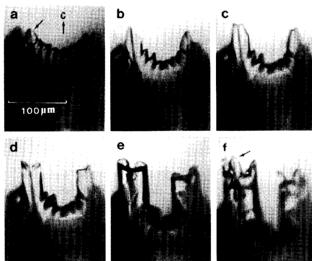
Fig. 5. Ice crystal growing in air at 10^5 Pa and at -7^\circ\text{C} and at about 10% (a–e) and about 13% (f) supersaturation. (a) 0, (b) 0.3, (c) 0.5, (d) 1.0, (e) 3.0 and (f) 4.0 min.
