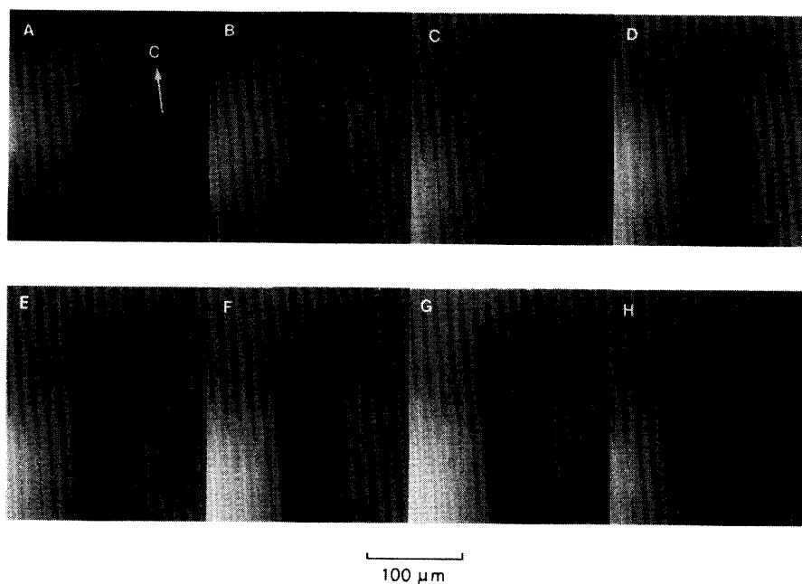
Fig. 6. Further growth of the secondary branch indicated by an arrow in Fig. 5f. (A) 0, (B) 0.5, (C) 1.0, (D) 1.5, (E) 2.0, (F) 2.5, (G) 3.0 and (H) 3.5 min.
