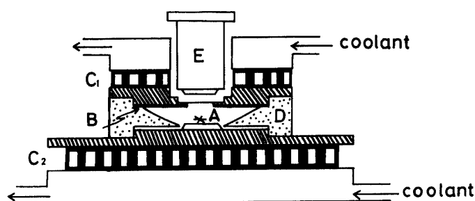
Fig. 1. Schematic diagram of a growth chamber.
