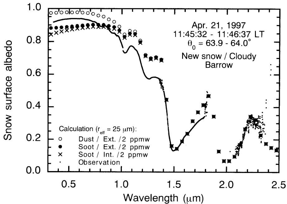
Fig. 5. Same as Fig. 4, except for theoretical results, which are calculated for r_{\text{eff}}=25 \mu\text{m} with soot-contaminated snow containing 2 ppmw internal mixture, soot-contaminated snow containing 2 ppmw external mixture and dust-contaminated snow containing 2 ppmw external mixture.
