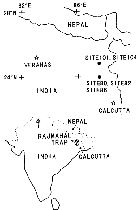
Fig. 1. Sampling location at Rajmahal trap. Solid circles show the sampling locality.
