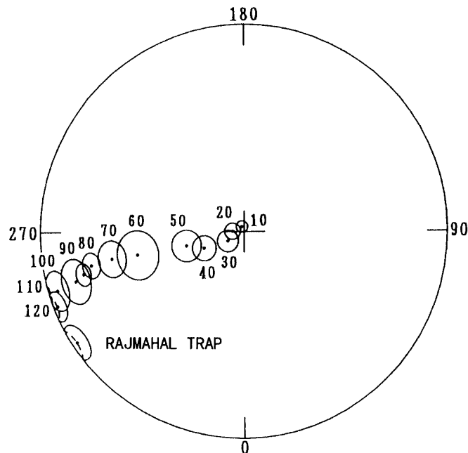
Fig. 5. VGP of Rajmahal trap plotted by equal-area net projection and APWP of India by BESSE and COURTILOT (1991).
