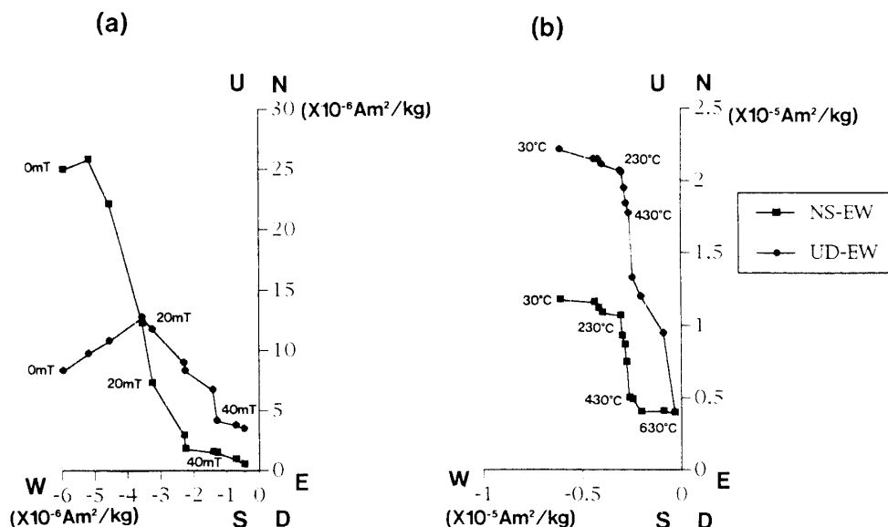
Fig. 3. Zijderveld graphs of AF and thermal demagnetization of NRM of the gneissic rocks from Skarvsnes. E: East, W: West, N: North, S: South, U: Up, D: Down (a) AF demagnetization (0–50 mT). (b) Thermal demagnetization ( 30^\circ\text{C} – 630^\circ\text{C} ).
