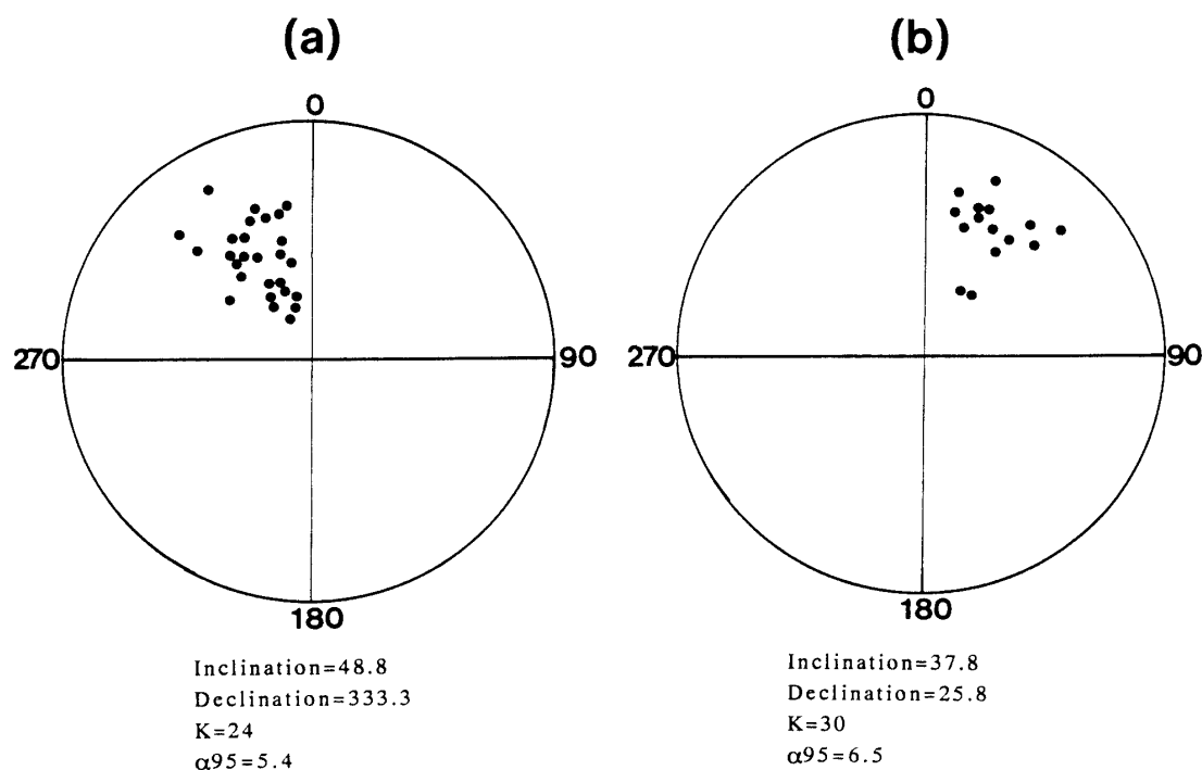
Fig. 6. The paleomagnetic results of the gneissic rocks from Skarvsnes area. (a) VGP: Lat. = 11.2^{\circ} S, Lon. = 16.0^{\circ} E (b) VGP: Lat. = 2.5^{\circ} S, Lon. = 63.2^{\circ} E
