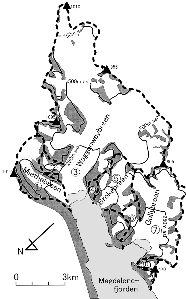
Fig. 6. Drainage basins of glaciers investigated at Magdalenefjorden. The glaciers are numbered for distinction (in circle), and the same numbers are used in Table 2, Fig. 7 and Fig. 8.
