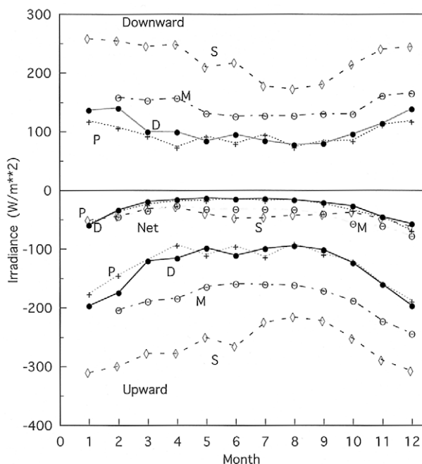
Fig. 3. Surface longwave radiation fluxes at Dome Fuji Station (D) in 1997, compared with those at three other Antarctic stations, Plateau (P; 1967), Mizuho (M; 1979) and Syowa (S; 1987).
