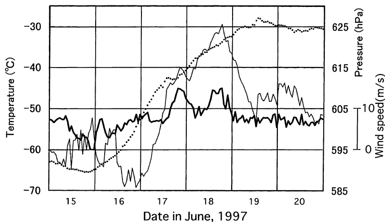
Fig. 5. Time series of surface air temperature (thin solid line), pressure (dotted line) and wind speed (thick solid line) at the surface of Dome Fuji Station during the abrupt warming in June 1997 (in LT; Hirasawa et al. , 2000).
