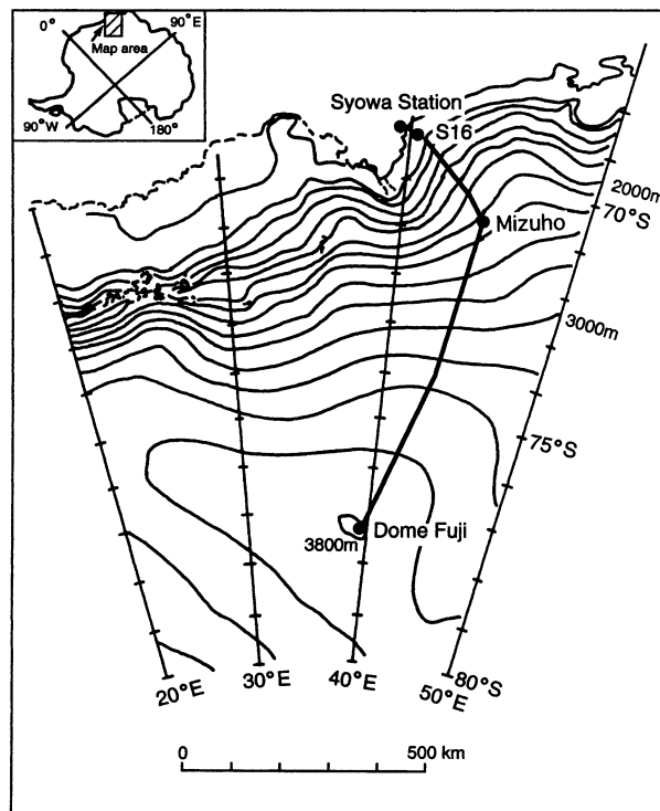
Fig. 1. Location of Dome Fuji Station.
