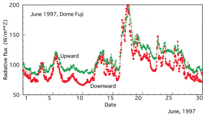
Fig. 7. Downward and upward longwave radiative fluxes at Dome Fuji Station in June 1997 (in LT).
