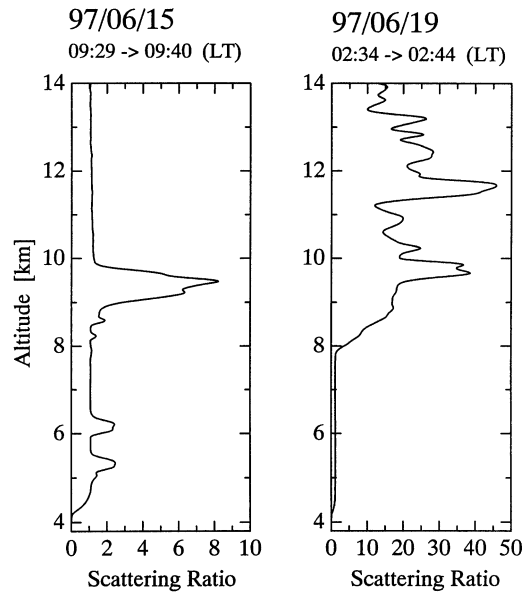
Fig. 9. Vertical profiles of lidar backscatter signal at Dome Fuji Station, 15 and 19 June 1997.
