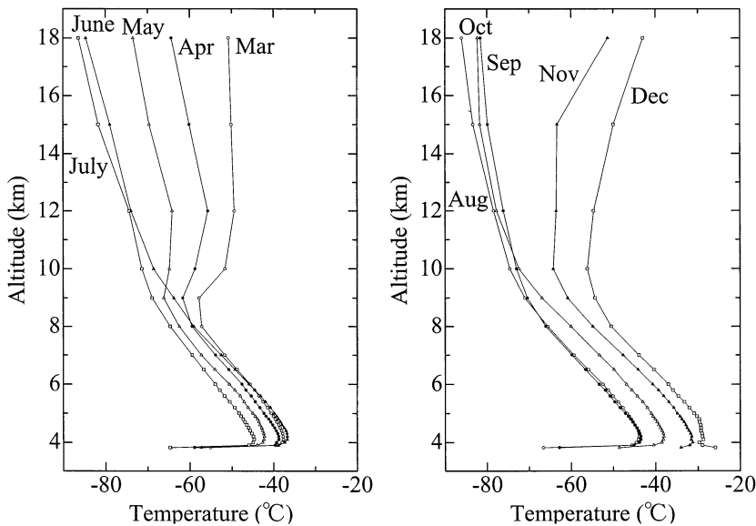
Fig. 4. Monthly mean temperature profiles at Dome Fuji Station from aerological soundings in 1997.
