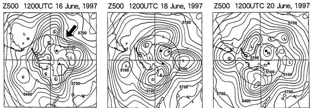
Fig. 6. 500 hPa geopotential height field for 1500 LT (1200 UTC) on 16, 18 and 20 June 1997, from Japan Meteorological Agency operational analysis (Hirasawa et al. , 2000). Locations of the Dome Fuji and Vostok Stations are indicated by a solid circle and triangle, respectively, and the blocking ridge is indicated by an arrow (16 June).
