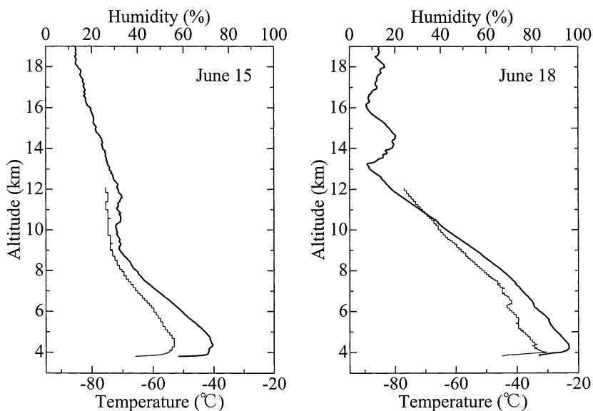
Fig. 8. Vertical profiles of temperature (thick line) and humidity (thin line) obtained by aerological sounding at Dome Fuji Station, 15 and 18 June 1997.
