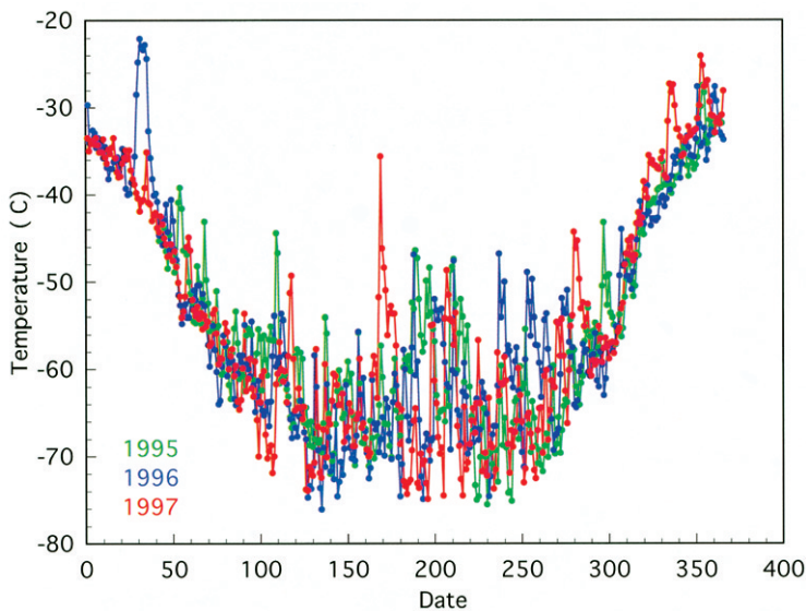
Fig. 2. Variations of daily temperature at Dome Fuji Station in 1995, 1996 and 1997.
