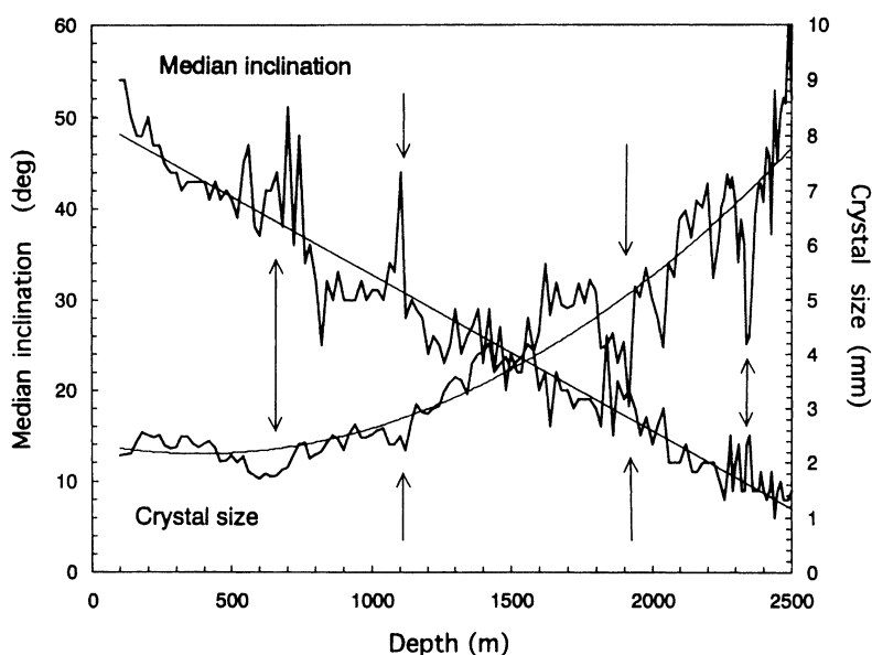
Fig. 2. Texture development of the Dome Fuji ice core (Azuma et al. , 2000).
