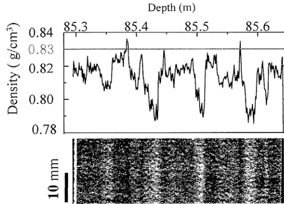
Fig. 3. X-ray density profile and x-ray stratigraphy (Hori et al. , 1999).
