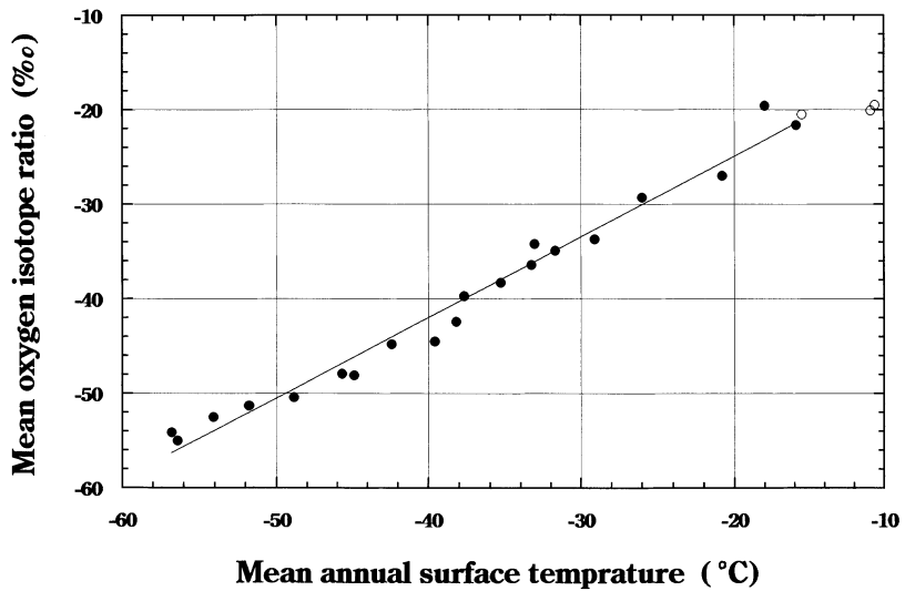
Fig. 3. Mean \delta^{18}\text{O} value of near-surface snow plotted against mean annual surface temperature (10 m-depth snow temperature) (after Satow et al. , 1999). The straight line is given by eq. (2). Three points on the coast marked by open circles are excluded from the regression equation.
