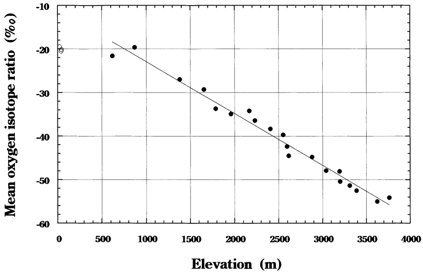
Fig. 2. Mean \delta^{18}\text{O} value of near-surface snow plotted against elevation (after Satow et al. , 1999). The straight line represents eq. (1).
