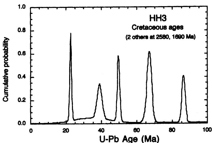
Fig. 8. Cumulative probability of SHRIMP zircon dating of pelitic granulite (HH3) from the Hidakhorobetsu River area. Data from WATANABE et al. (1997; in prep. ).
