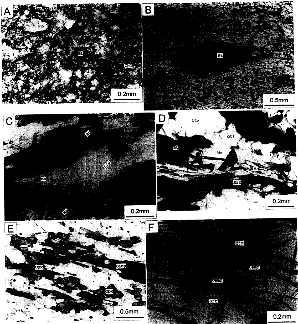
Fig. 4. Photomicrographs of metamorphic rocks in the study area. A: Meta-graywacke from the lower biotite zone. B: Spotted slate from the upper biotite zone. C: Biotite-muscovite schist from the upper biotite zone. D: Biotite-muscovite-fibrolite gneiss from the sillimanite-muscovite zone. E: Orthoamphibole-bearing rock from the orthopyroxene zone. F: Orthoamphibole inclusions in garnet in the same sample as E.
