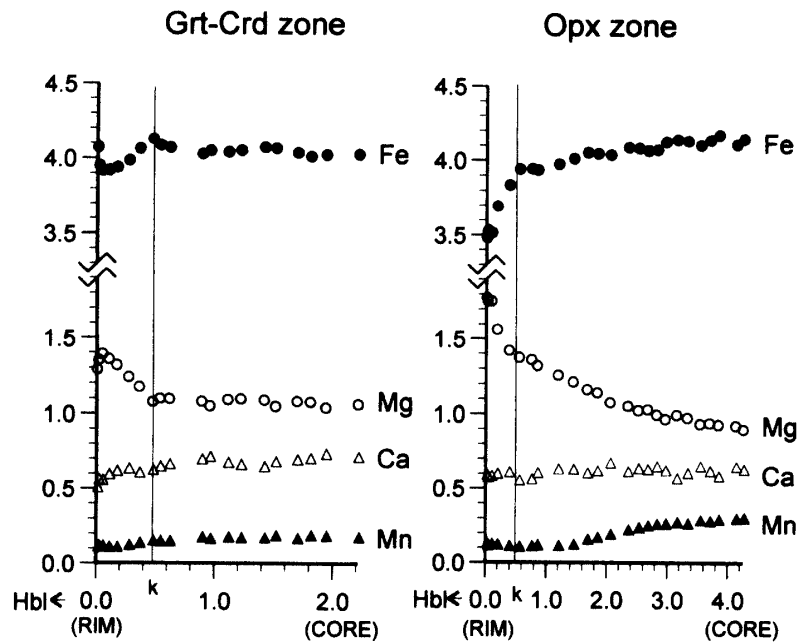
Fig. 7. Rim-core zoning profiles from garnets in amphibolite from the Grt-Crd and Opx zones. Fe, solid circles; Mg, open circles; Ca, open triangles; Mn, solid triangles. Profiles plotted in cations per formula unit based on 24 oxygens. X-axis indicates the distance from the rim in mm. "k" indicates a kink in the profiles. Mineral in immediate contact with garnet is also shown.
