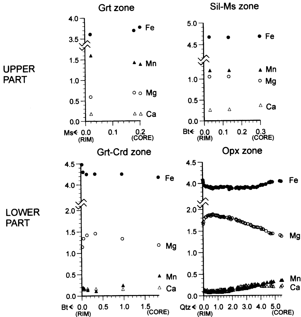
Fig. 6. Rim-core zoning profiles from garnets in pelitic rocks from each metamorphic zone. Fe, solid circles; Mg, open circles; Ca, open triangles; Mn, solid triangles. Profiles plotted in cations per formula unit based on 24 oxygens. X-axis indicates the distance from the rim in mm. Minerals in immediate contact with garnet are also shown.
