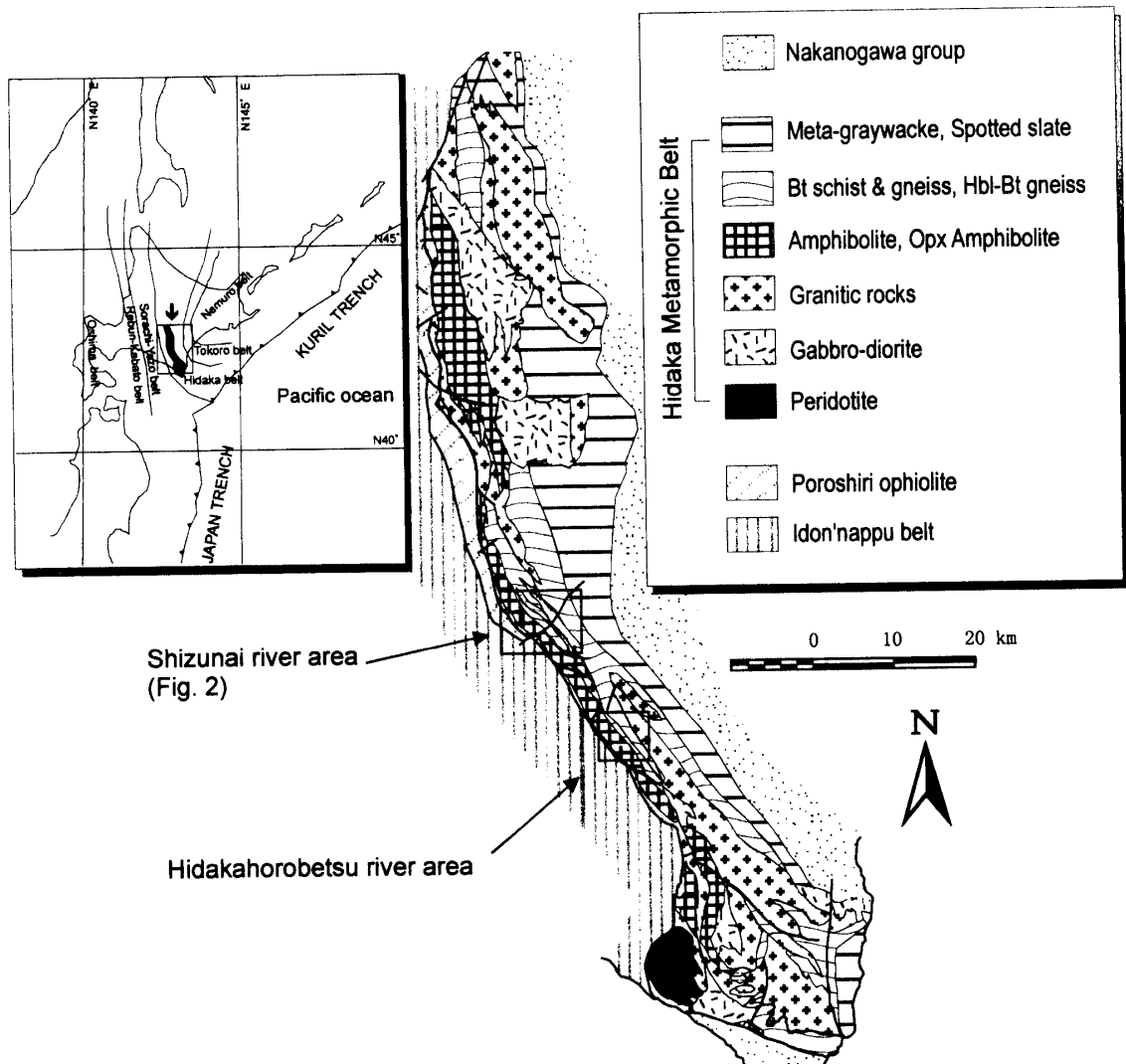
Fig. 1. Simplified geological map of the Hidaka Metamorphic Belt (KOMATSU et al. , 1989). The tectonic division of Hokkaido is modified from KIMIMAMI et al. (1986).
