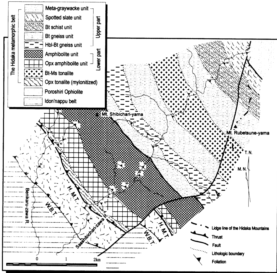
Fig. 2. Geological map of the Shizunai River area (modified from the map by OSANAI, 1985).
