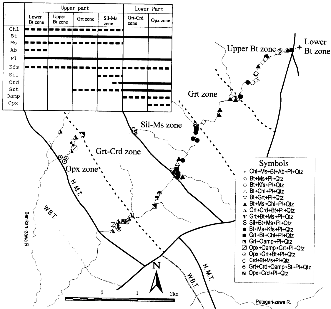
Fig. 3. Map showing distribution of mineral assemblages in pelitic and orthoamphibole-bearing rocks in the Shizunai River area. Stabilities of minerals in each zone are shown in the inset. Solid line: major constituent; dashed line: minor constituent. Abbreviation of minerals after KRETZ (1983), except Oamp (orthoamphibole).
