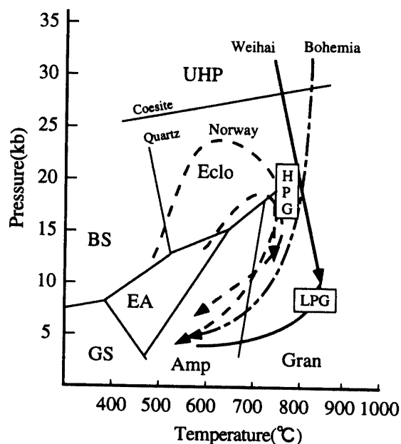
Fig. 13. Reported P - T paths for granulite facies overprinting on the UHP/HP rocks inset metamorphic facies boundaries are same as those in Fig. 6. HPG: high pressure granulite, LPG: low-pressure granulite.
