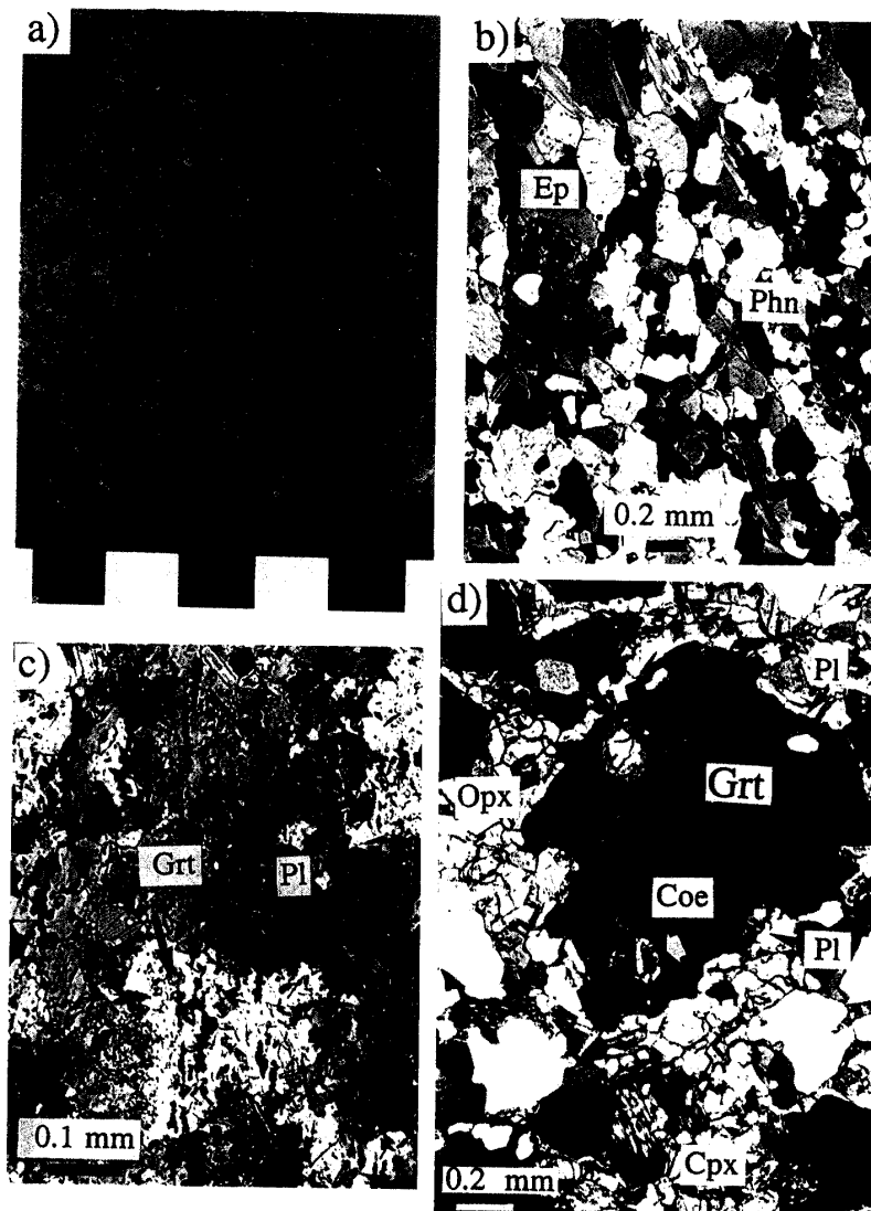
Fig. 12. Representative photo/photomicrograph of the streaky gneiss and the Su-Lu gneiss at Yangkou, and of the coesite-bearing granulite at Weihai. a) Polished surface of the Su-Lu gneiss (94YK32). b) Photomicrograph of the quartz-feldspar-rich layer of the Su-Lu gneiss (94YK32). Phn: phengite, Ep: epidote. Crossed nicols. c) Annealing texture of the streaky gneiss (92YK2). Foliation defined by fine-grained garnet (Grt) is overgrown by plagioclase (Pl). Crossed nicols with test plate. d) Photomicrograph of the coesite (Coe)-bearing Weihai granulite. Cpx: clinopyroxene, Opx: orthopyroxene, Pl: plagioclase.
