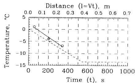
Fig. 5. Temperature of EWS: solid line is outer surface of the core barrel, dashed line is inner surface; l=0 is the bottom of the drilling bit.
