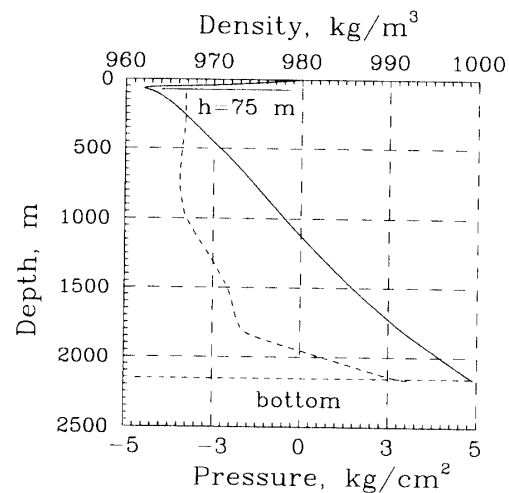
Fig. 8. Density of EWS (dashed line) and pressure difference (solid line) between EWS and ice-overburden pressure in a hypothetical borehole; H is level of EWS in the borehole.
