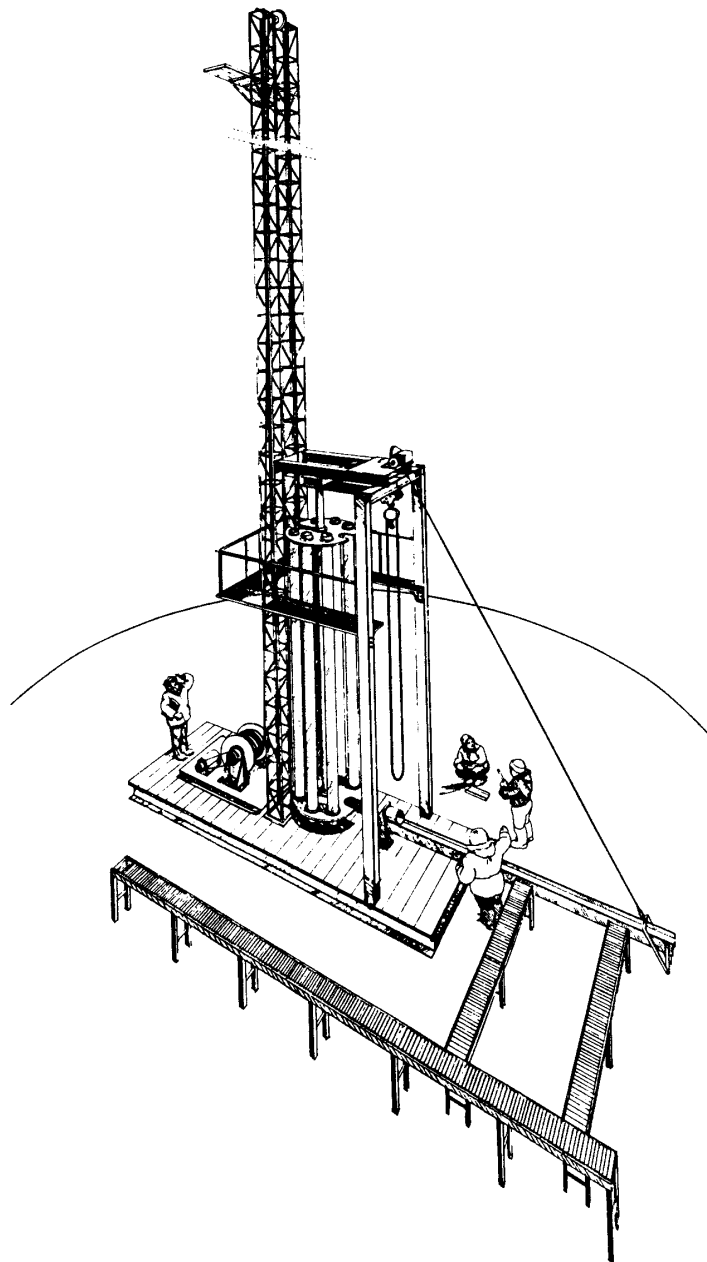
Fig. 1. PICO 13.2 cm ice core drill handling system.
