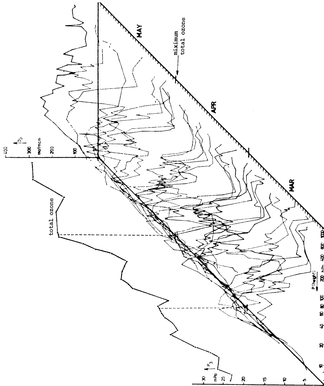
Fig. 2b. Lindenbergl, March, April and May 1985.
