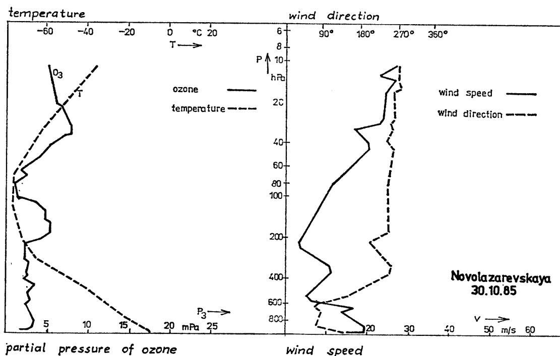
Fig. 1d. Novolazarevskaya, October 30, 1985.
