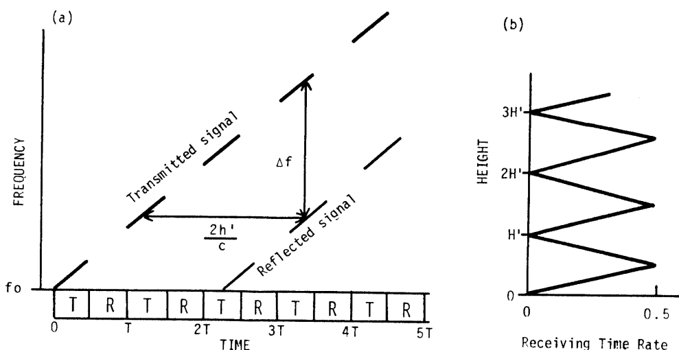
Fig. 1. Concept of pulsed FM/CW (pulsed chirp) method. a. Frequency-time representation of signals. Frequency swept signal is transmitted with the period of T and reflected signal is taken in by the receiver only in receiving windows (time interval indicated by R ). b. The reception time rate with layer height h' for the fixed pulse period of T=2H'/c .
