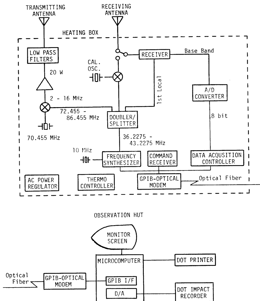
Fig. 3. Block diagram of the system.
