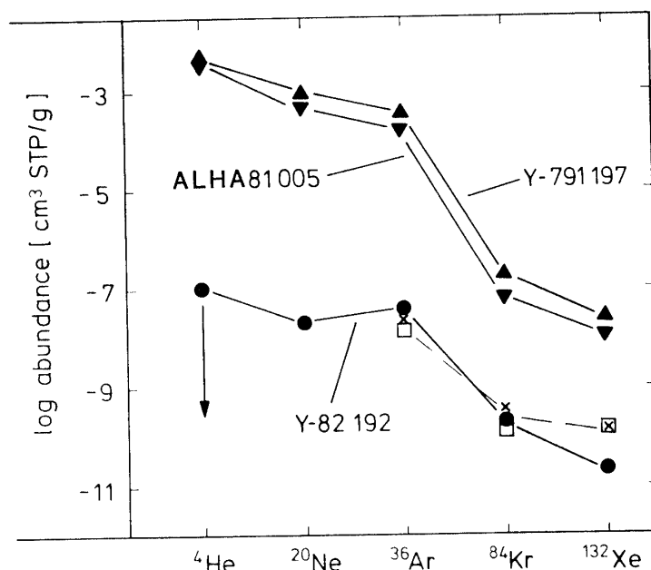
Fig. 9. Nuclide abundance patterns of trapped noble gases in three lunar meteorites. In Y-791197 and ALHA81005 the abundances of all nuclides except He are very similar to those in the lunar regolith. (In the present plot Y-791197 and lunar regolith would be indistinguishable except for ^4\text{He} which is about 7 times higher in the regolith (TAKAOKA, 1986). Y-82192, on the other hand, is much more similar to normal chondrites of high petrologic grade (□) and to the Apollo XVII boulder (shown are the results (×) for the anorthositic breccia (LEICH et al. , 1975).
