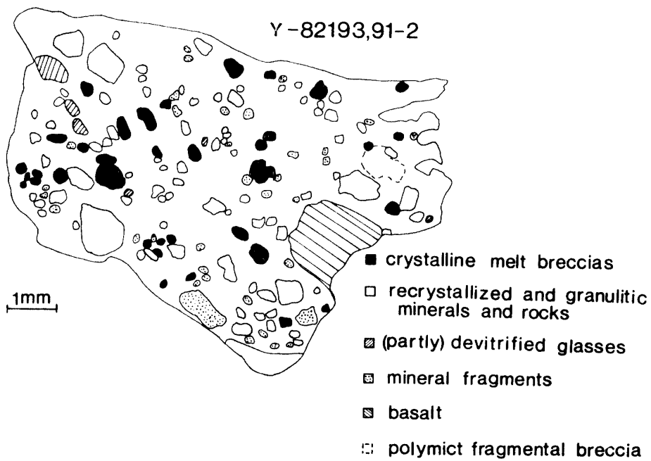
Fig. 2. Sketch map of thin section Y-82193,91-2 showing the distribution of mineral and lithic clasts.
