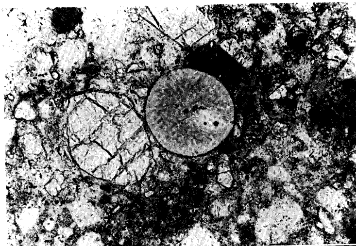
Fig. 6a. Y-82192: a recrystallized spherule ( \sim 130 \mu\text{m} in apparent diameter) is embedded in a fine-grained matrix; one polarizer.
