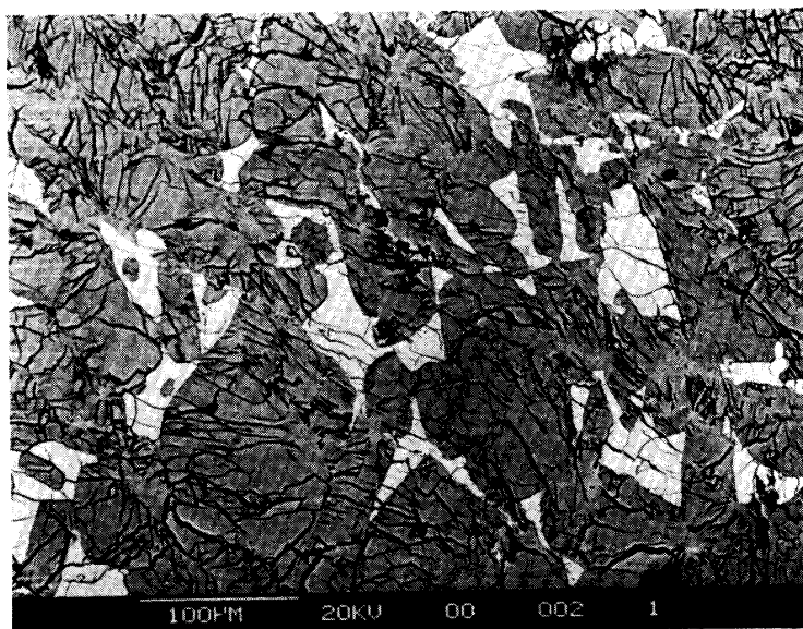
Fig. 7. Microstructure of a basaltic clast in Y-82193 consisting of pyroxene (light) and plagioclase (dark gray). Image in backscattered electrons.
