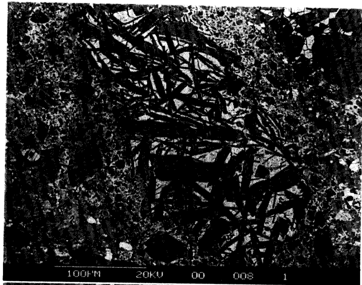
Fig. 5. Crystalline impact melt breccias: plagioclase (dark gray), mafic minerals (light gray); images in backscattered electrons.
