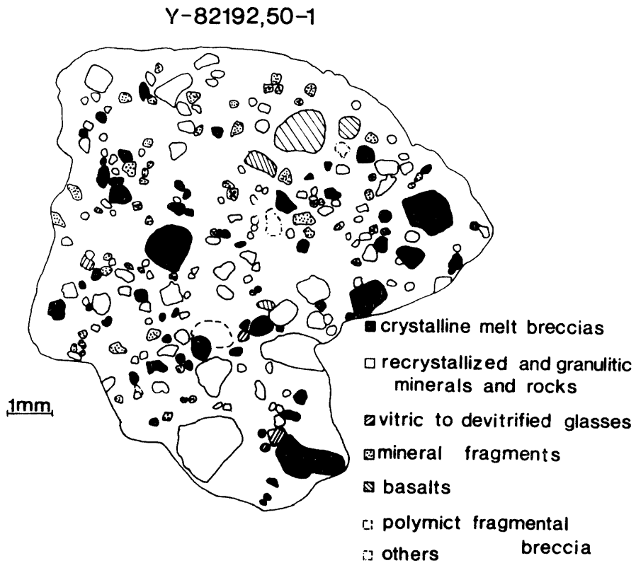
Fig. 1. Sketch map of thin section Y-82192,50-1 showing the distribution of mineral and lithic clasts.
