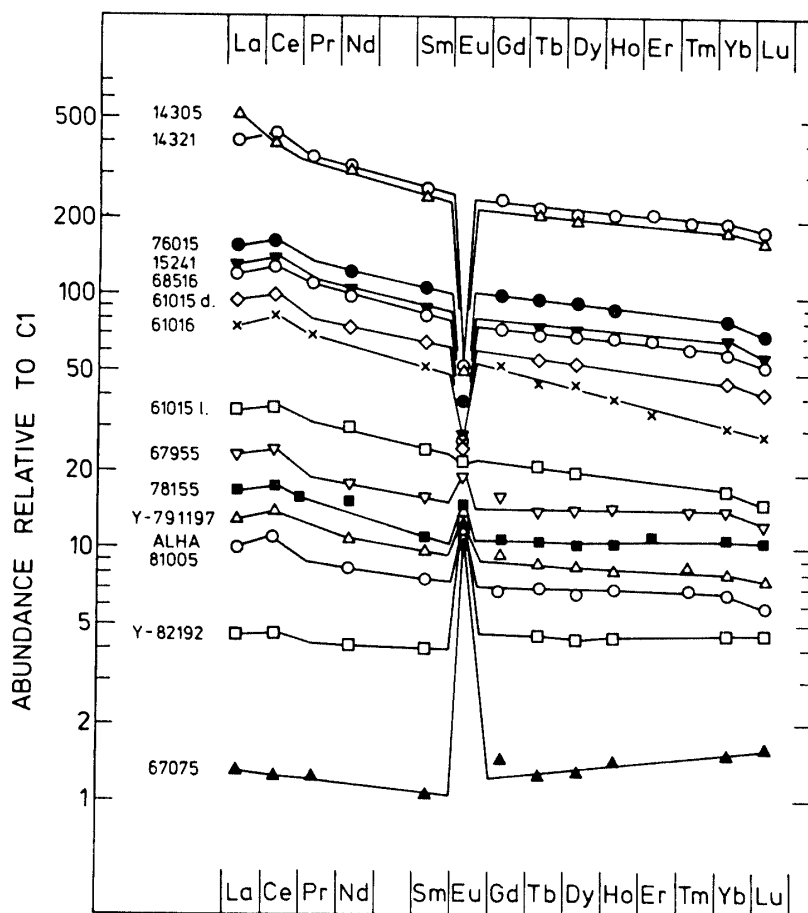
Fig. 8. CI-normalized REE-abundances of lunar highland samples and three lunar meteorites. The parallel patterns of Apollo 14, 16, and 17 rocks are due to the presence of a KREEP component. The patterns for 67955, 78155, and ALHA81005 are slightly different with their flat HREE. Y-791197 could have a small amount of KREEP. But in Y-82192 the KREEP component is completely lacking. Data for ALHA81005 and Y-791197 from PALME et al. (1983) and OSTERTAG et al. (1986). Data for lunar highland rocks are from the Mainz laboratory.
