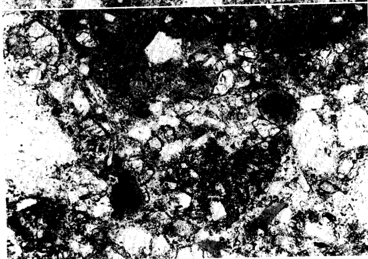
Fig. 6b. Y-82193: a small recrystallized spherule ( \sim 100 \mu\text{m} in apparent diameter) and a devitrified impact glass (lower left); one polarizer.
