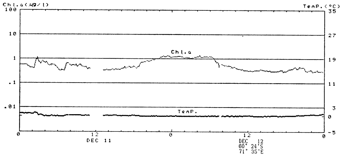
Fig. 6. Time serial records of the surface chlorophyll a and temperature between 0000 LT December 11 and 0000 LT December 13, 1984 in the westward course on the southward leg.
