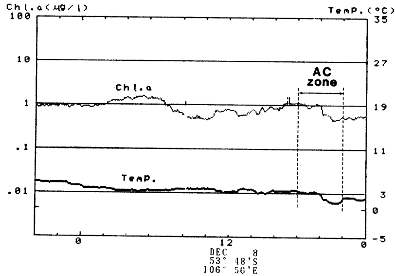
Fig. 5. Time serial records of the surface chlorophyll a and temperature between 2000 LT December 7 and 0000 LT December 9, 1984 on the southward leg across the Antarctic Convergence (AC) zone.
