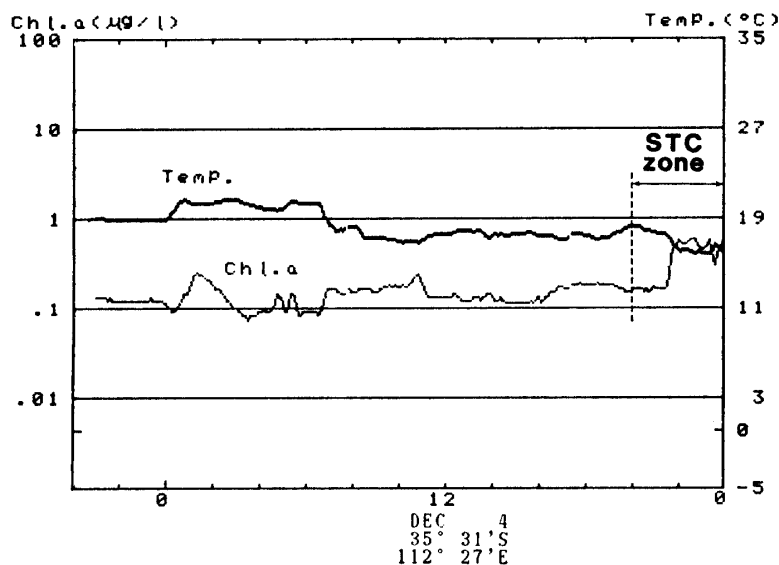
Fig. 3. Time serial records of surface chlorophyll a and temperature between 2000 LT December 3 and 0000 LT December 5, 1984 on the southward leg across the Subtropical Convergence (STC) zone.
