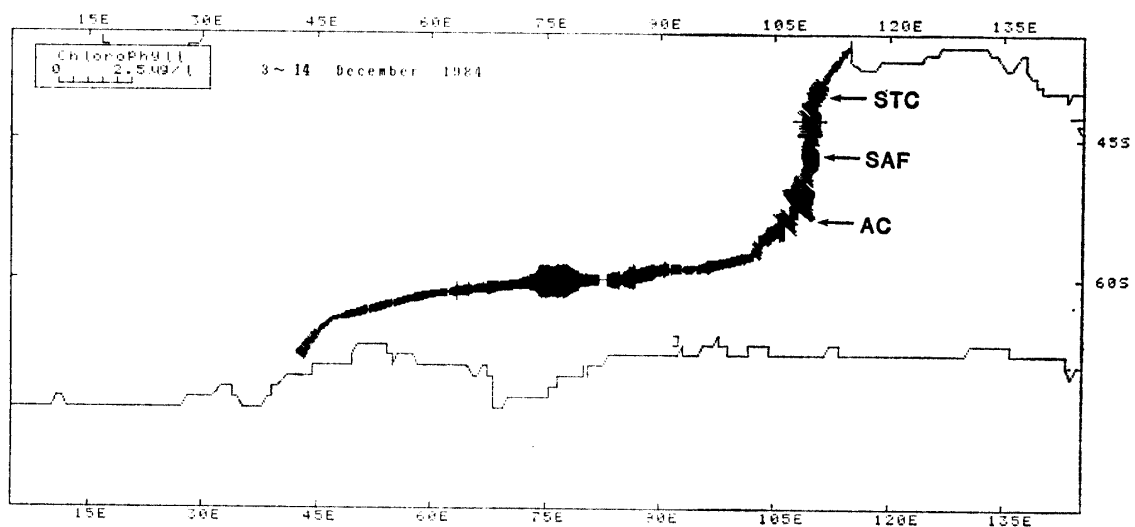
Fig. 2. Horizontal distribution of chlorophyll a in the surface water (8 m depth) along the course of the southward leg of icebreaker SHIRASE between 3 and 14 December 1984. AC, SAF and STC indicate approximate locations of the Antarctic Convergence, Subantarctic Front and Subtropical Convergence.
