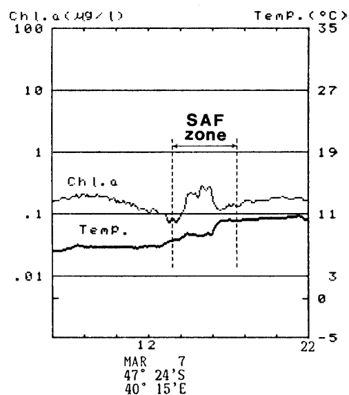
Fig. 8. Time serial records of the surface chlorophyll a and temperature between 0600 LT March 7 and 0000 LT March 8, 1985 on the northward leg across the Subantarctic Front (SAF) zone.
