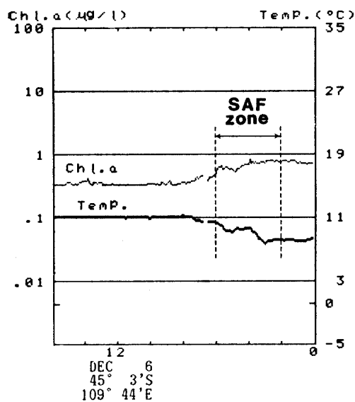
Fig. 4. Time serial records of surface chlorophyll a and temperature between 0800 LT December 6 and 0000 LT December 7, 1984 on the southward leg across the Subantarctic Front (SAF) zone.
