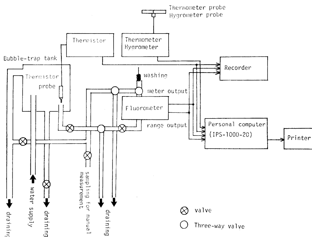
Fig. 1. Schematic representation of the continuous measuring-recording system of the surface chlorophyll a employed for the JARE-26 (1984/85).
