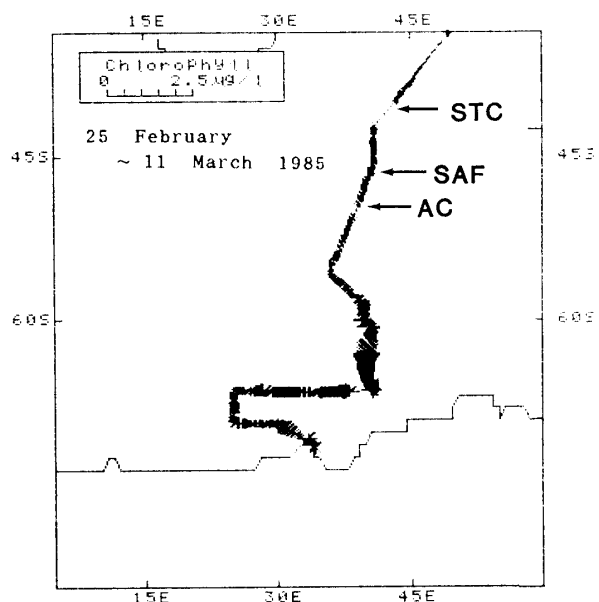
Fig. 7. Horizontal distribution of chlorophyll a in the surface water (8 m depth) on the northward leg along the course of icebreaker SHIRASE between 25 February and 11 March 1985. AC, SAF and STC as in Fig. 2.
