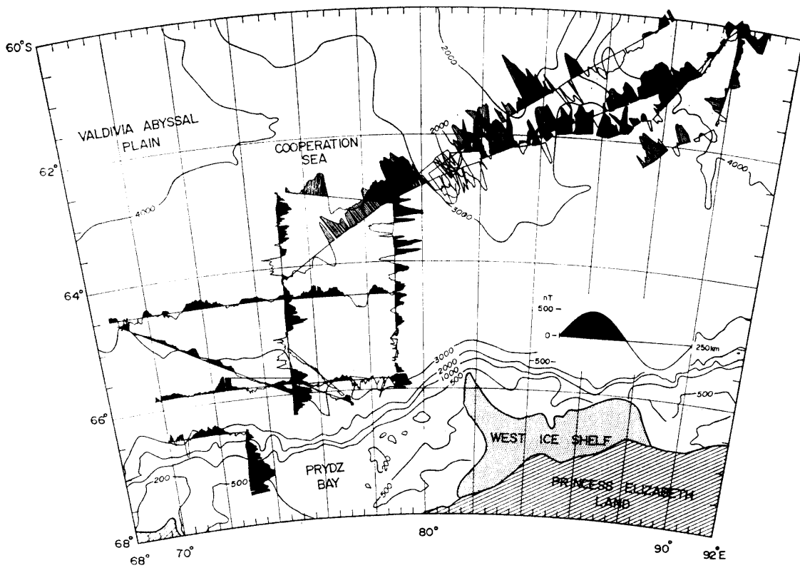
Fig. 4. Magnetic anomaly profiles along the vessel tracks. Reference field: IGRF1980.
