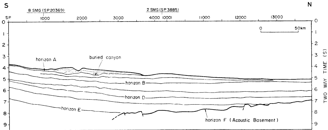
Fig. 7. Interpreted section of line 4 SMG.
