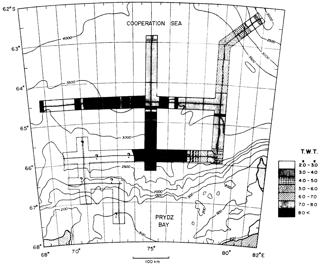
Fig. 12. Schematic acoustic basement map of two-way travel time (s) off the Amery Ice Shelf. The acoustic basement cannot be identified in the continental shelf and slope because of sea bottom multiple reflections.
