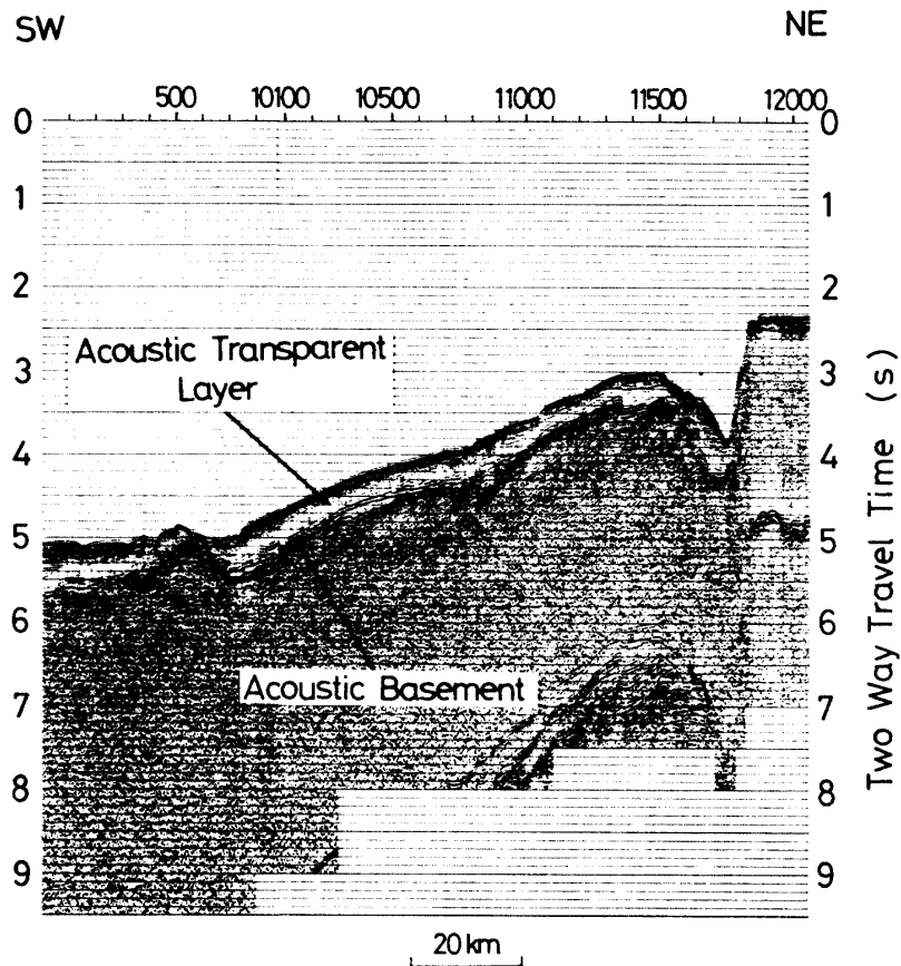
Fig. 9. Seismic profile of line 12 SMG. Dipping reflections are identified in the acoustic basement between S.P. 10500 and S.P. 11500.
