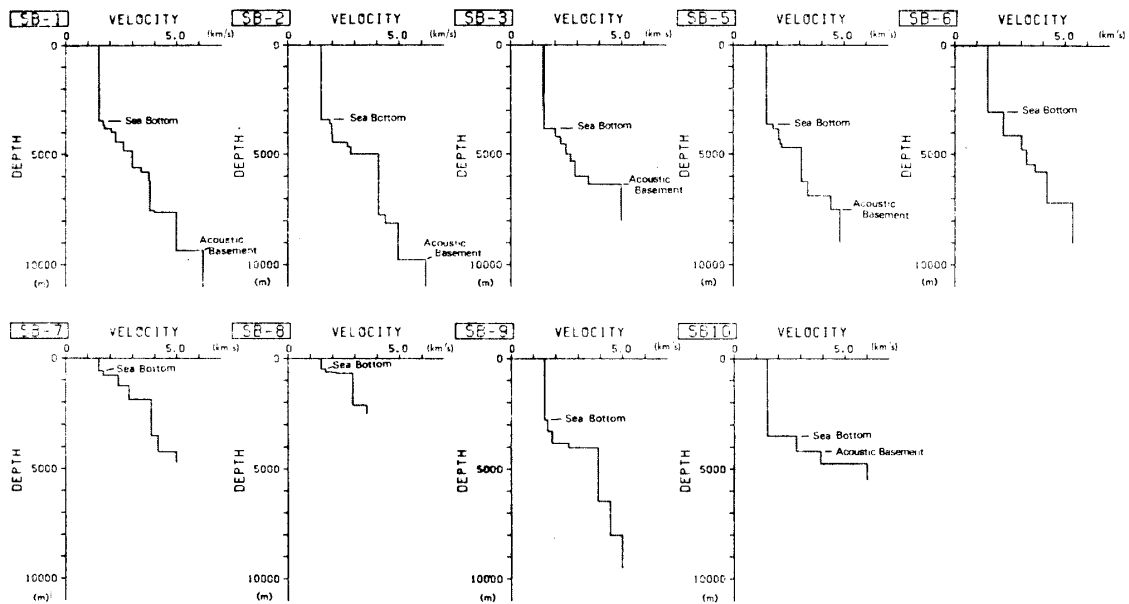
Fig. 10. Velocity-depth profiles derived from sonobuoy survey.
