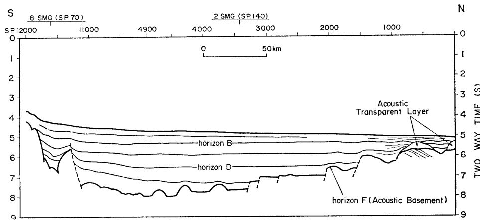
Fig. 8. Interpreted section of line 7 SMG.
