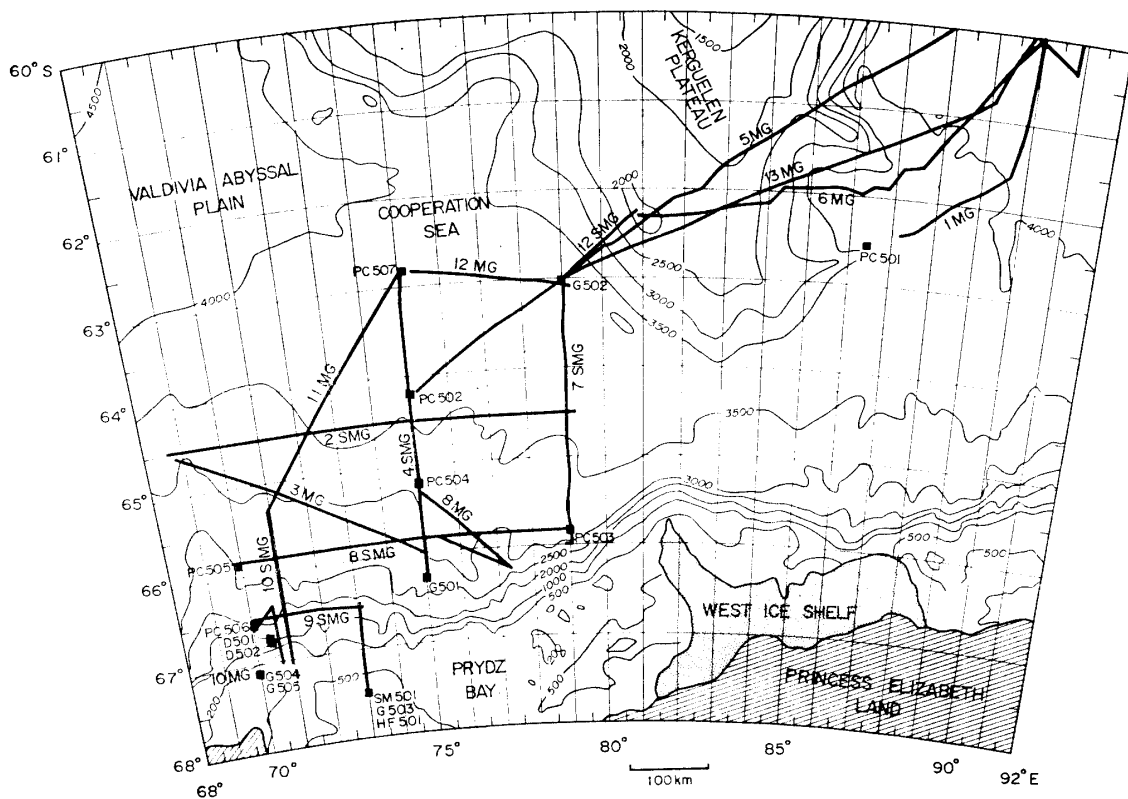
Fig. 2. Lines of geophysical survey and sampling stations off the Amery Ice Shelf. SMG: seismic, magnetic, gravity; MG: magnetic, gravity; PC: piston core; G: gravity core; D: dredge; SM: Smith-McIntyre grab; HF: heat flow.
