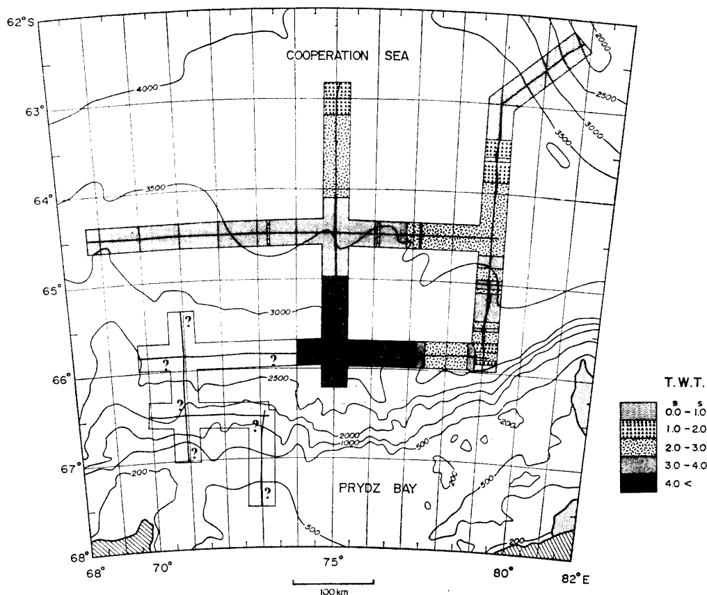
Fig. 13. Schematic isochron map of total sediments in seconds off Amery Ice Shelf.
