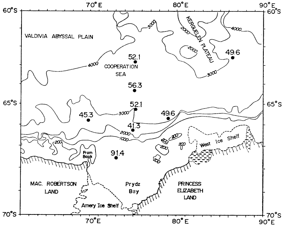
Fig. 11. Terrestrial heat flow distribution off the Amery Ice Shelf (unit; mW/m^2 ).
