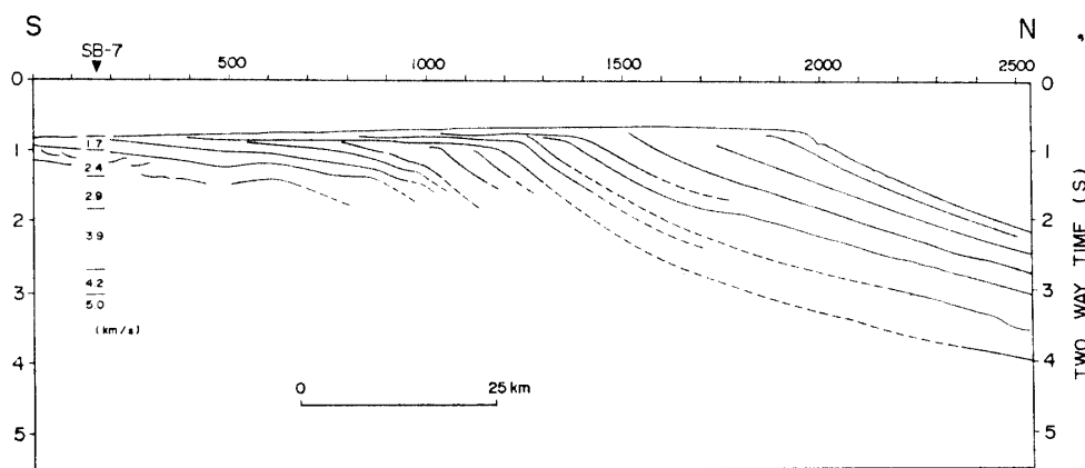
Fig. 6. Interpreted section of line 9 SMG.
