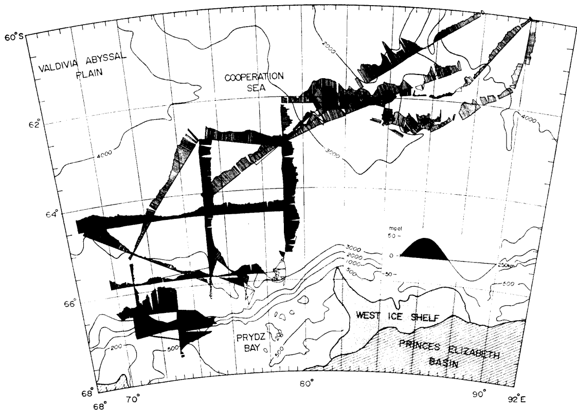
Fig. 3. Free-air gravity anomaly profiles along the vessel tracks. Reference field: IGSN71.
