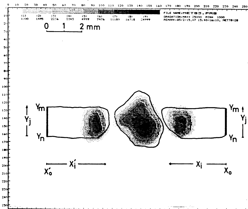
Fig. 3b. Spatial distribution of natural thermoluminescence for slices in pair and for interior one.
