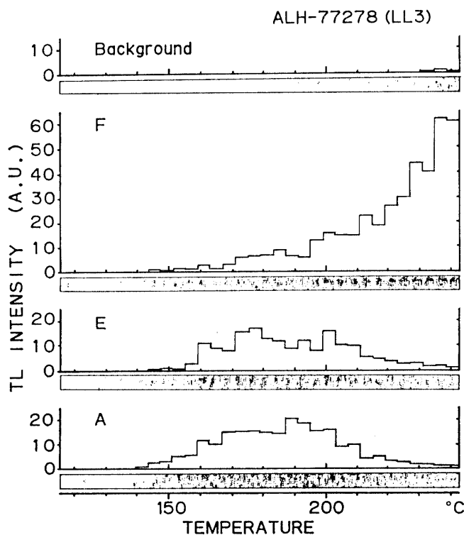
Fig. 4c. Glow curve of chondrules.
