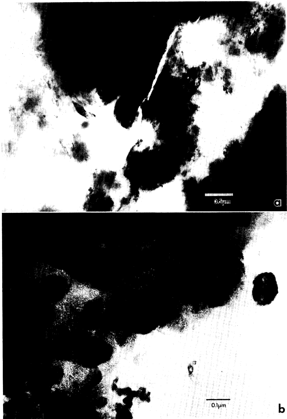
Fig. 6. Electron micrograph indicating matrix textures in Y-791198. a. In this region, phyllosilicates are aggregated. b. In the figure, FeS grains are aggregated.
