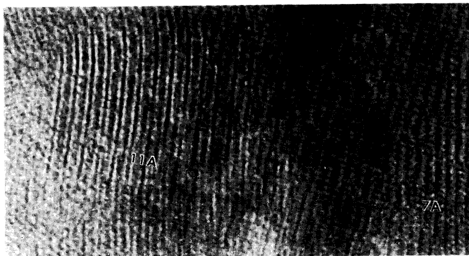
Fig. 10. Electron micrograph of 11Å layer mineral in Y-791198 which were recently supposed to be tochilinite (MACKINNON and ZOLENSKY, 1984). It is grown in parallel intergrowth with 7Å platy phyllosilicate.
