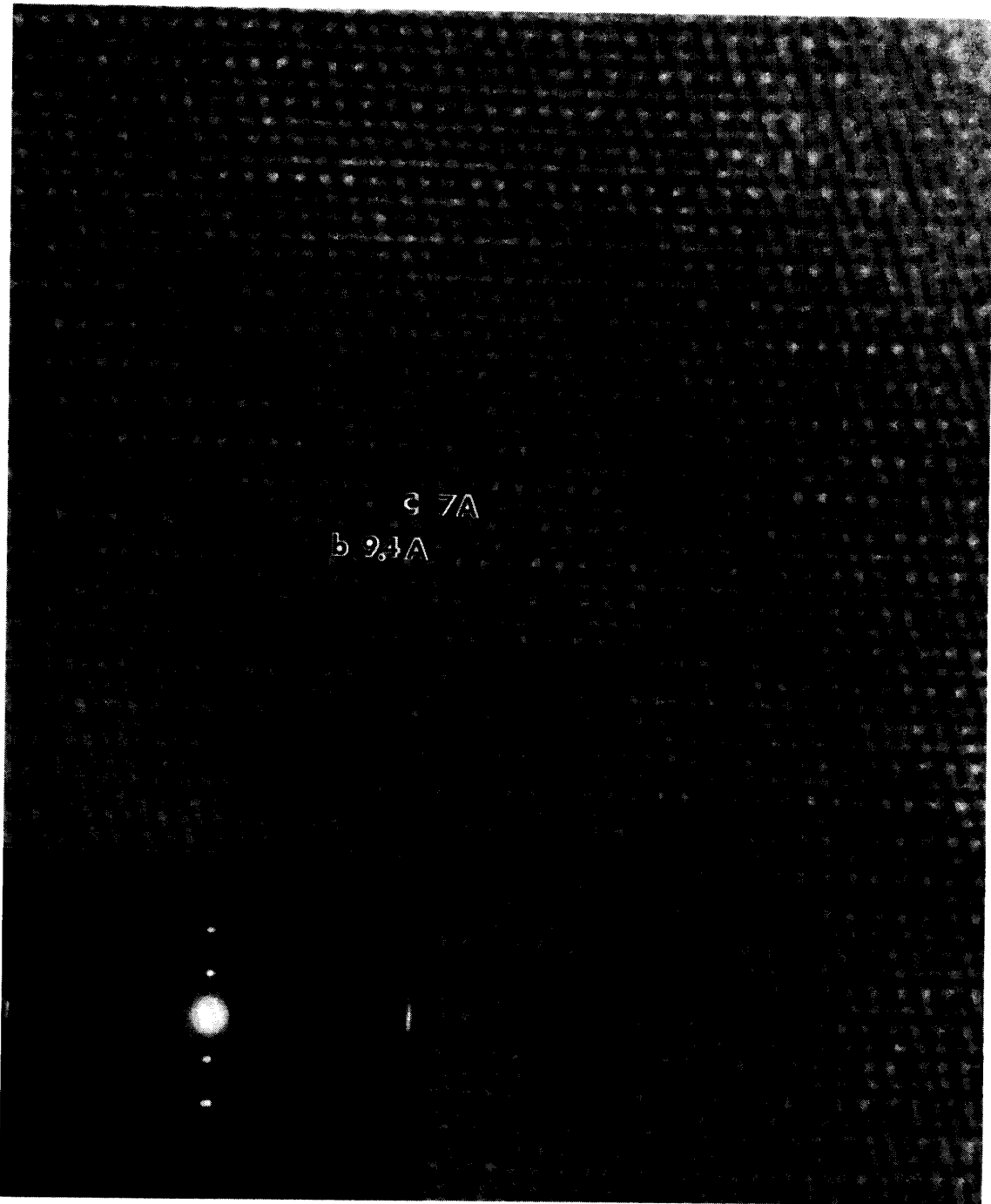
Fig. 9. High resolution electron micrograph of stacking disorder in 7Å thick platy phyllosilicate (Y-791198).
