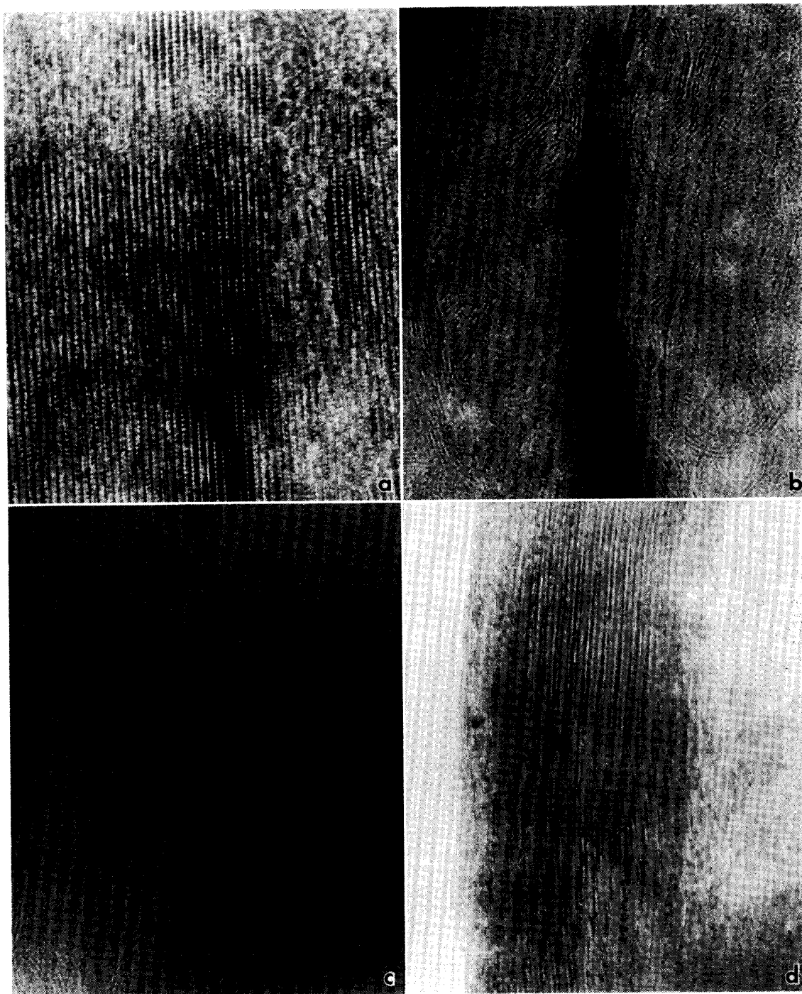
Fig. 8. Electron micrographs of matrix phyllosilicate types in Y-791198.
