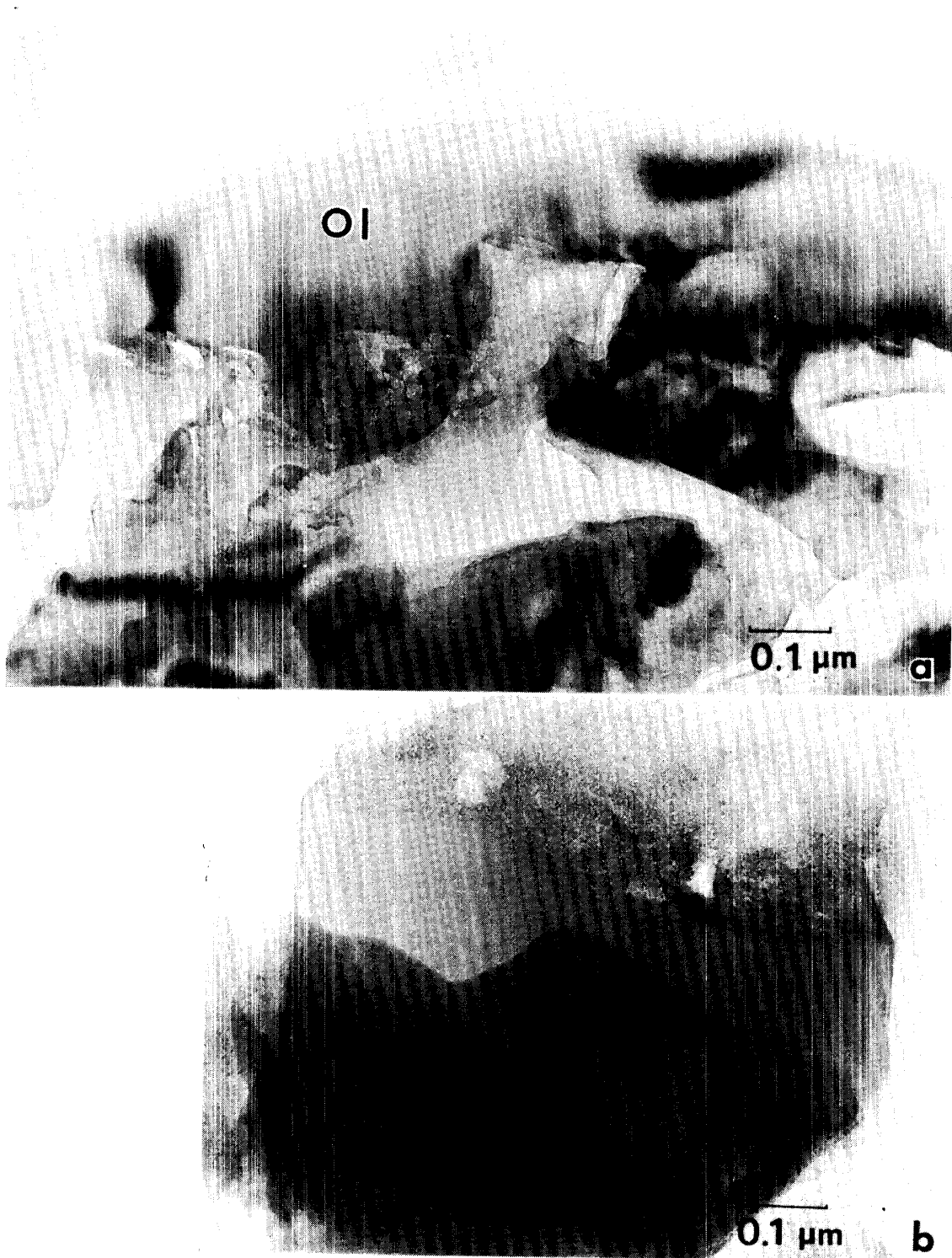
Fig. 7. Electron micrograph indicating matrix mineral grains (a: forsterites) whose shapes appear as if they were corroded by some fluid phase (Y-791198).
