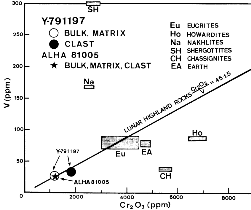
Fig. 3. V vs. Cr 2 O 3 correlation in moon, earth and achondrite bodies. The data are taken from DREIBUS et al. (1978), SMITH (1982), LAUL et al. (1972, 1983). The Y-791197 data fall on the lunar highland line. This correlation for the moon samples was first noted by LAUL et al. (1972).
