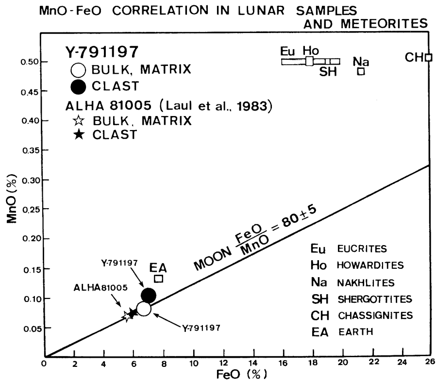
Fig. 1. MnO vs. FeO correlation in moon, earth and achondrite bodies. The lunar FeO/MnO ratio of 80 \pm 5 first noted by LAUL et al. (1972) is characteristic of the moon and provides strong evidence in favor of a lunar origin for Y-791197.
