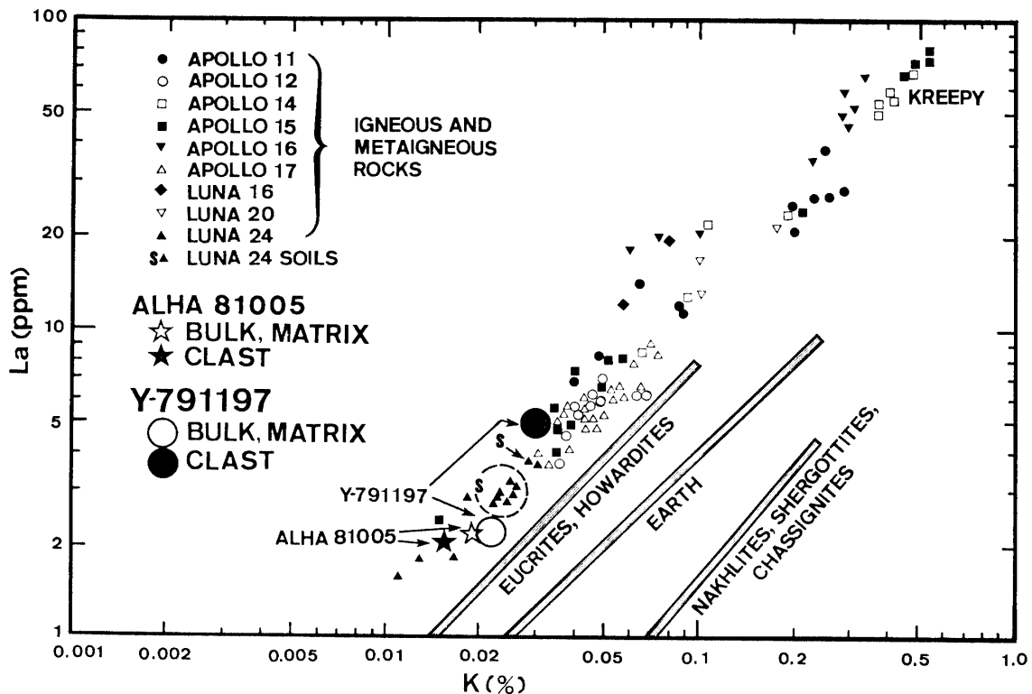
Fig. 2. K vs. La correlation in moon, earth and achondrite bodies. This correlation was first noted by WÄNKE et al. (1973). The data for earth and achondrites are taken from WÄNKE and DREIBUS (1982).
