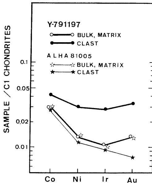
Fig. 5. C1 chondrites (non-volatile) normalized abundance patterns of siderophiles in bulk, matrix and clast of Y-791197 and ALHA81005 meteorites. The later data are taken from LAUL et al. (1983).
