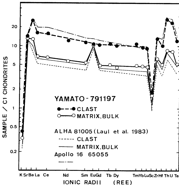
Fig. 4. C1 chondrites (non-volatile) normalized abundance patterns of the large-ion lithophile (LIL) elements in bulk, matrix and clast of Y-791197 and ALHA81005 meteorites, and Apollo 16 65055 highland rock. The 65055 data are taken from TAYLOR (1982).
