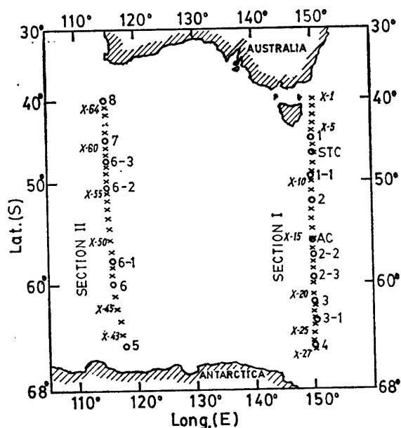
Fig. 1. Oceanographic stations and sections of the KH-83-4 cruise of the HAKUHO MARU during a period from December 11, 1983 to January 31, 1984. Open circles and crosses show CTDO and XBT stations, respectively.
