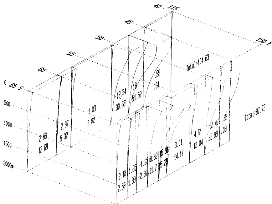
Fig. 9. Perspective diagram showing the geostrophic flow relative to 2000 db. Upper numeric: geostrophic velocity at surface (cm/s). Lower numeric: volume transport ( 10^6\text{m}^3/\text{s} ).
