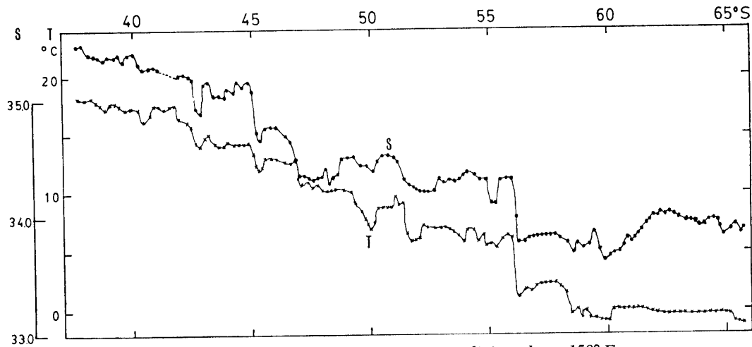
Fig. 4a. Sea surface temperature and salinity along 150°E.
