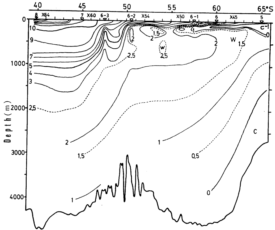
Fig. 2b. Vertical section of temperature ( ^{\circ}\text{C} ) along 115^{\circ}\text{E} .
