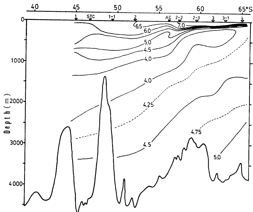
Fig. 6a. Vertical section of dissolved oxygen (ml/l) along 150°E.
