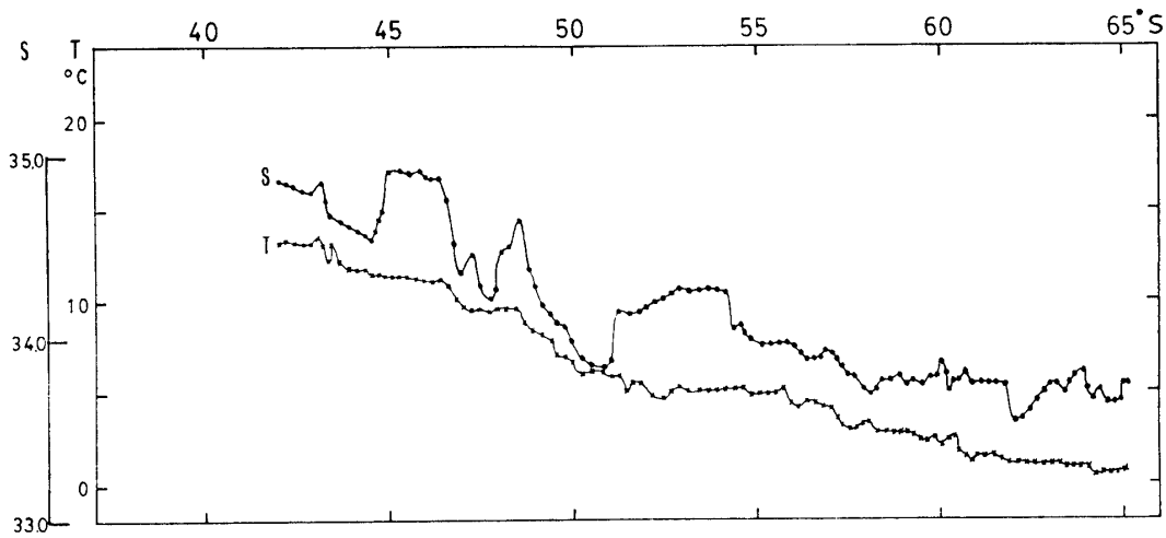
Fig. 4b. Sea surface temperature and salinity along 115°E.
