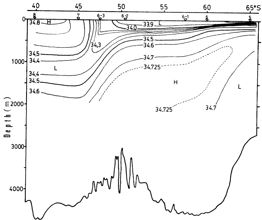
Fig. 3b. Vertical section of salinity along 115^{\circ}\text{E} .
