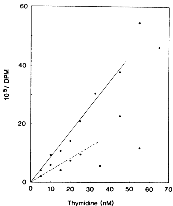
Fig. 5. Plots of reciprocal of [methyl- ^3\text{H} ] thymidine incorporation into TCA insoluble fraction. Closed circle: Stn. 2; open circle: Stn. 4.
