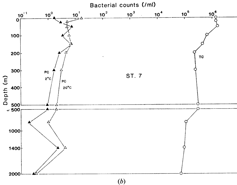
Fig. 2. Vertical profiles of bacterial counts at Stn. 5 (Fig. 2a) and Stn. 7 (Fig. 2b). TC: total counts, PC: plate counts.
