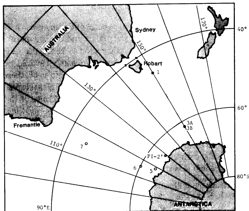
Fig. 1. Sampling locations during KH-83-4 cruise of R. V. HAKUHO MARU.
