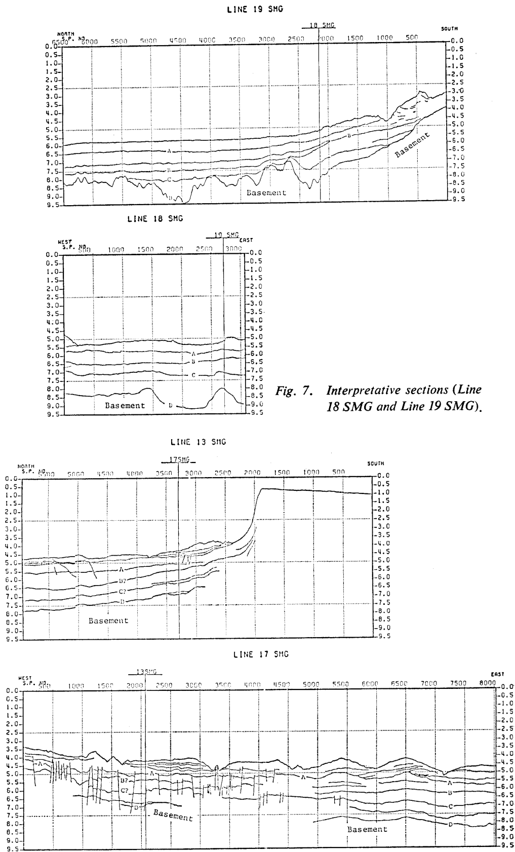
Fig. 8. Interpretative sections (Line 13 SMG and Line 17 SMG).
