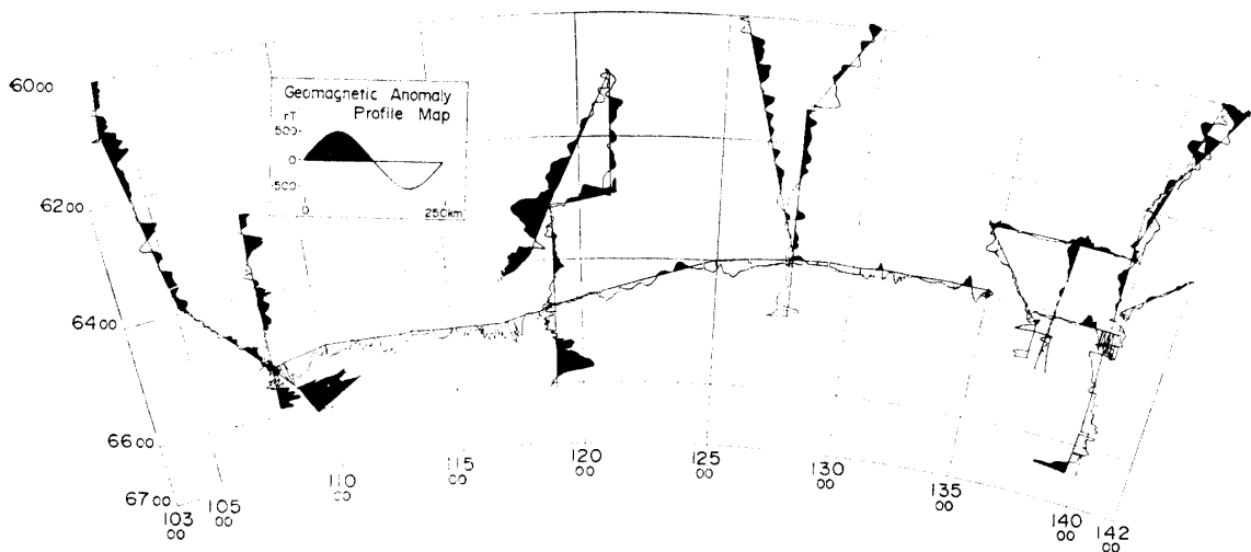
Fig. 15. Magnetic anomaly profile.
